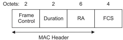
Figure 18—ACK frame
