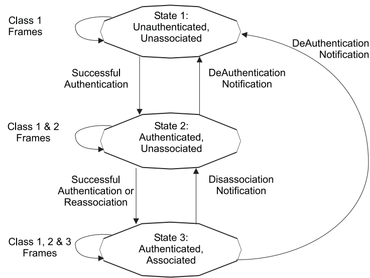
Figure 8—Relationship between state variables and services
