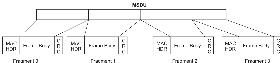
Figure 48—Fragmentation
