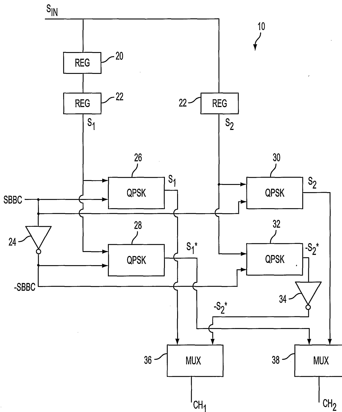
FIG. 3 (PRIOR ART)
