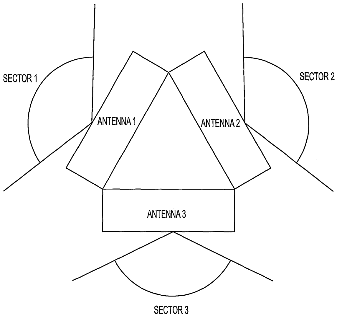
FIG. 8 (PRIOR ART)
