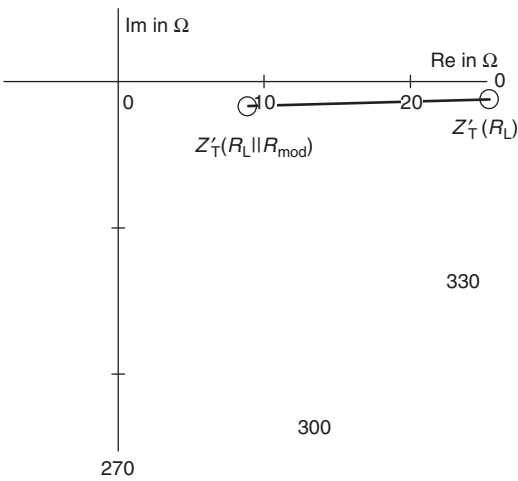
Figure 4.38 Locus curve of the transformed transponder impedance with ohmic load modulation ( R_L || R_{mod} = 1.5\text{--}5\text{ k}\Omega ) of an inductively coupled transponder. The parallel connection of the modulation resistor R_{mod} results in a lower value of Z'_T
