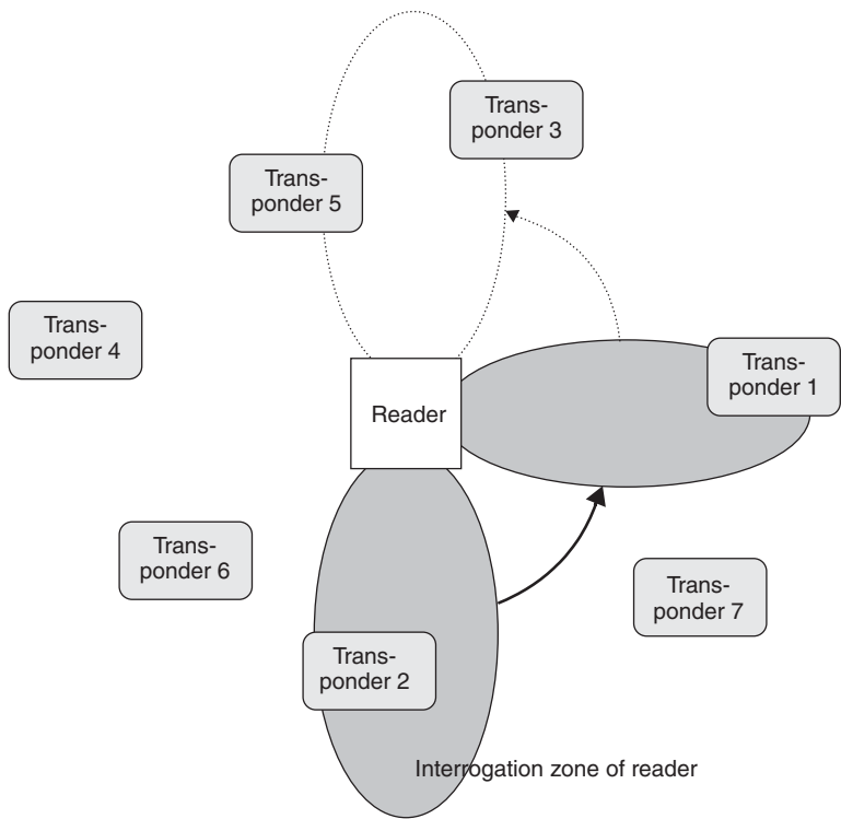
Figure 7.11 Adaptive SDMA with an electronically controlled directional antenna. The directional beam is pointed at the various transponders one after the other
