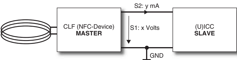
Figure 11.34 The single wire protocol transmits signals S1 and S2 represented by the voltage and current in a single wire
