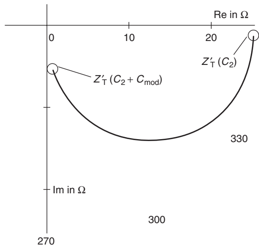
Figure 4.41 Locus curve of transformed transponder impedance for the capacitive load modulation ( C_2||C_{mod} = 40\text{--}60\text{ pF} ) of an inductively coupled transponder. The parallel connection of a modulation capacitor C_{mod} results in a modulation of the magnitude and phase of the transformed transponder impedance Z'_T
