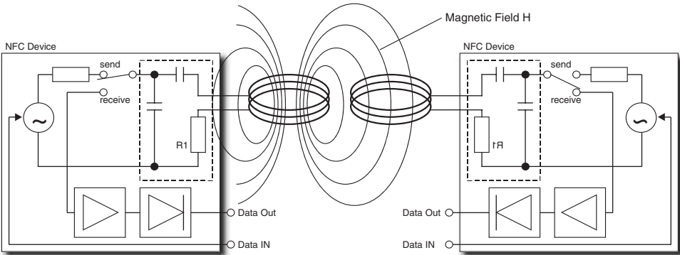
Figure 3.32 In active mode, the NFC interfaces alternately emit magnetic fields for data transmission
