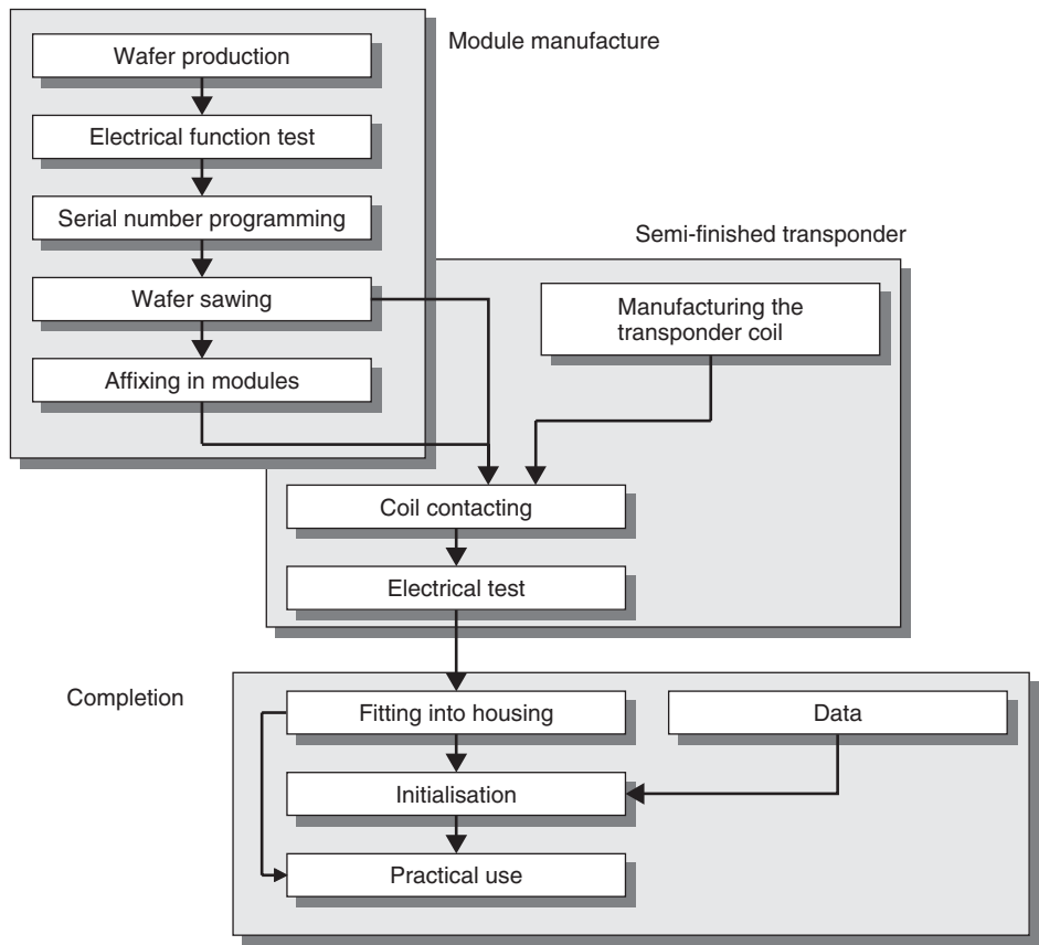
Figure 12.1 Transponder manufacture
