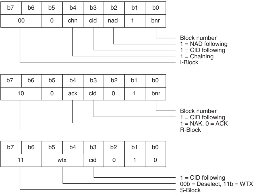
Figure 9.29 Coding of the PCB byte in a frame. The entire transmission behaviour is controlled by the PCB (protocol control byte) in the protocol
