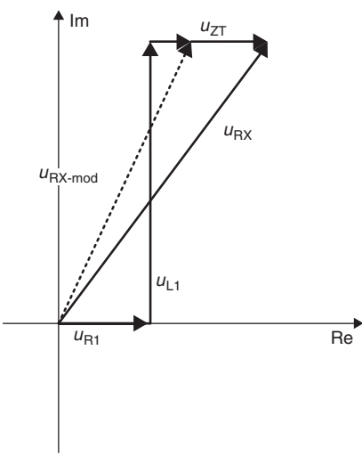
Figure 4.39 Vector diagram for the total voltage u_{RX} that is available to the receiver of a reader. The magnitude and phase of u_{RX} are modulated at the antenna coil of the reader ( L_1 ) by an ohmic load modulator
