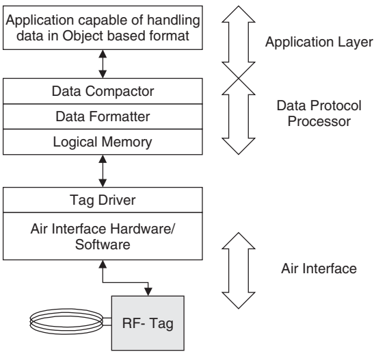
Figure 9.44 A command passes through several hardware and software layers specified by the existing standards
