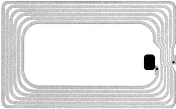
Figure 12.11 Example of a 13.56 MHz smart card coil using screen printing technology
