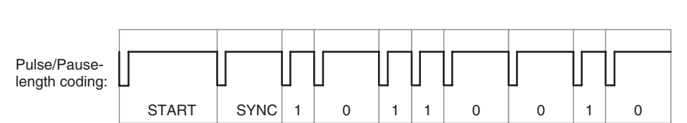
Figure 6.3 Possible signal path in pulse-pause coding
