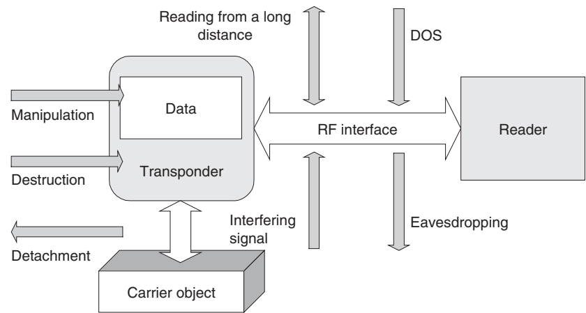
Figure 8.2 Some basic attack options on RFID systems (according to Rikcha, 2004)
