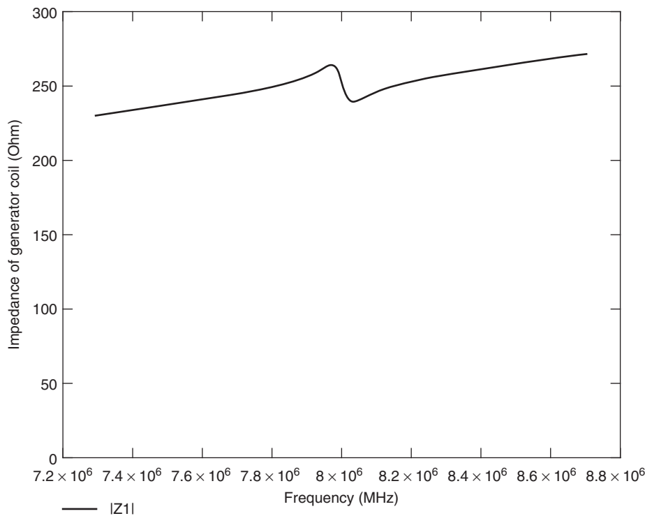
Figure 3.3 The occurrence of an impedance ‘dip’ at the generator coil at the resonant frequency of the security element ( Q = 90, k = 1\% ). The generator frequency f_G is continuously swept between two cut-off frequencies. An RF tag in the generator field generates a clear dip at its resonant frequency f_R
