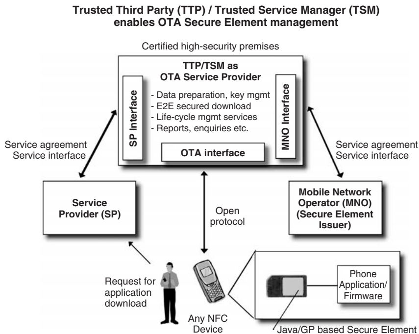
Figure 13.14 Administration of the secure element of an NFC-enabled phone via OTA service (Yliutinen, 2007; figure Venyon)
