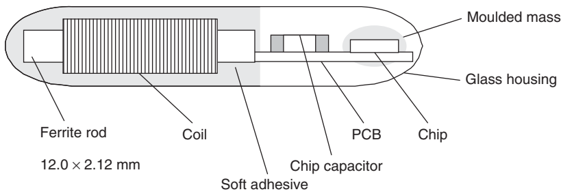
Figure 2.4 Mechanical layout of a glass transponder
