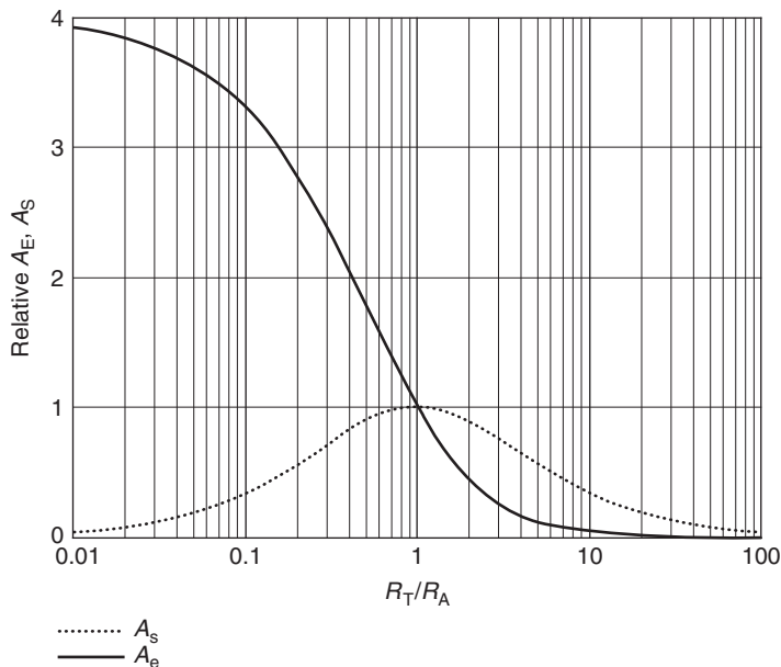
Figure 4.67 Graph of the relative effective aperture A_e and the relative scatter aperture \sigma in relation to the ratio of the resistances R_A and R_r . Where R_T/R_A = 1 the antenna is operated using power matching ( R_T = R_r ). The case R_T/R_A = 0 represents a short-circuit at the terminals of the antenna
