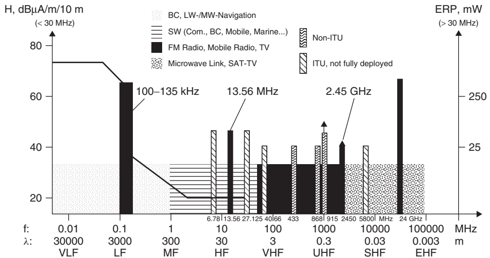
Figure 5.1 The frequency ranges available for RFID systems range from the myriametric range below 135 kHz, through short wave and ultrashort wave to the microwave range, with the highest frequency being 24 GHz. In the frequency range above 135 kHz the ISM bands available worldwide are preferred
