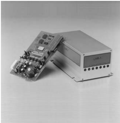
Figure 11.27 Example of an OEM reader for use in terminals or robots (photo: long-range/high-speed reader LHRI, reproduced by permission of SCEMTEC Transponder Technology GmbH, Reichshof-Wehnrath)
