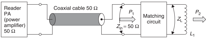
Figure 11.21 Connection of an antenna coil using 50 \Omega technology
