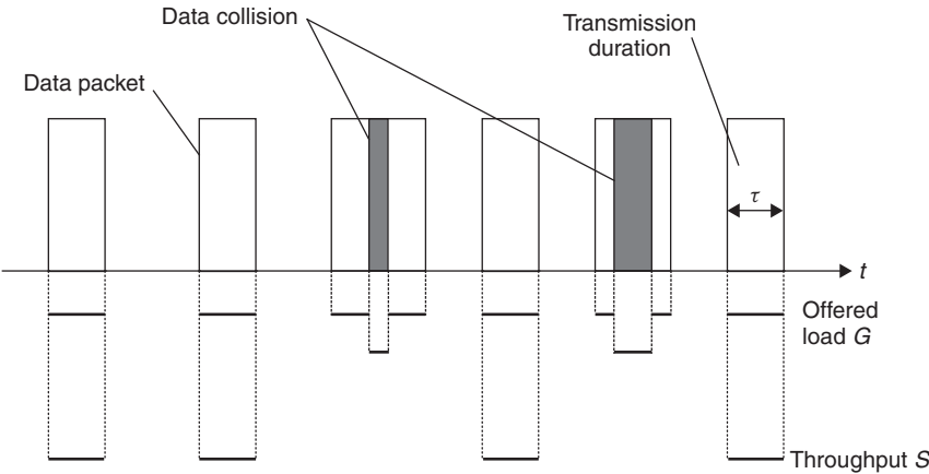
Figure 7.14 Definition of the offered load G and throughput S of an ALOHA system: several transponders send their data packets at random points in time. Now and then this causes data collisions, as a result of which the (data) throughput S falls to zero for the data packets that have collided
