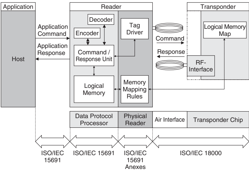
Figure 9.43 Relation between different standards of the ISO 18000 series
