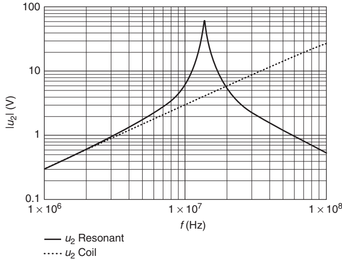
Figure 4.14 Plot of voltage at a transponder coil in the frequency range 1–100 MHz, given a constant magnetic field strength H or constant current i_1 . A transponder coil with a parallel capacitor shows a clear voltage step-up when excited at its resonant frequency ( f_{\text{RES}} = 13.56\text{ MHz} )
