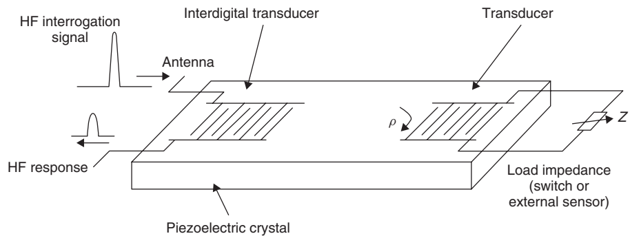
Figure 4.105 Principal layout of a passive surface wave transponder connected to an external sensor (reproduced by permission of Siemens AG, ZT KM, Munich)
