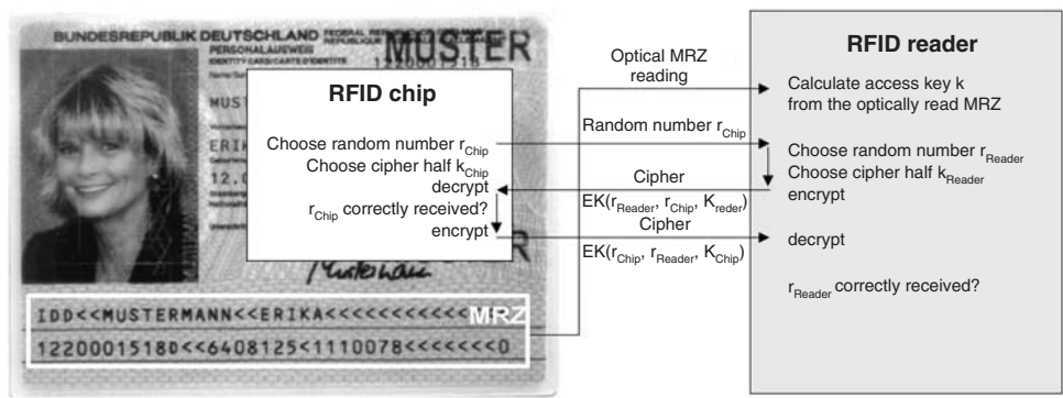
Figure 13.21 Basic access control simulates the behaviour of current passports
