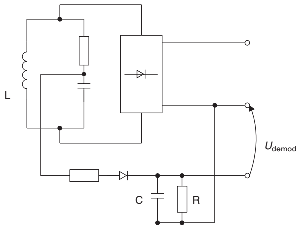
Figure 10.6 A 100 % ASK modulation can be simply demodulated by an additional diode
