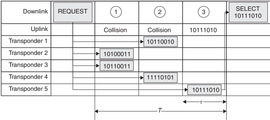
Figure 7.17 Transponder system with slotted ALOHA anticollision procedure
