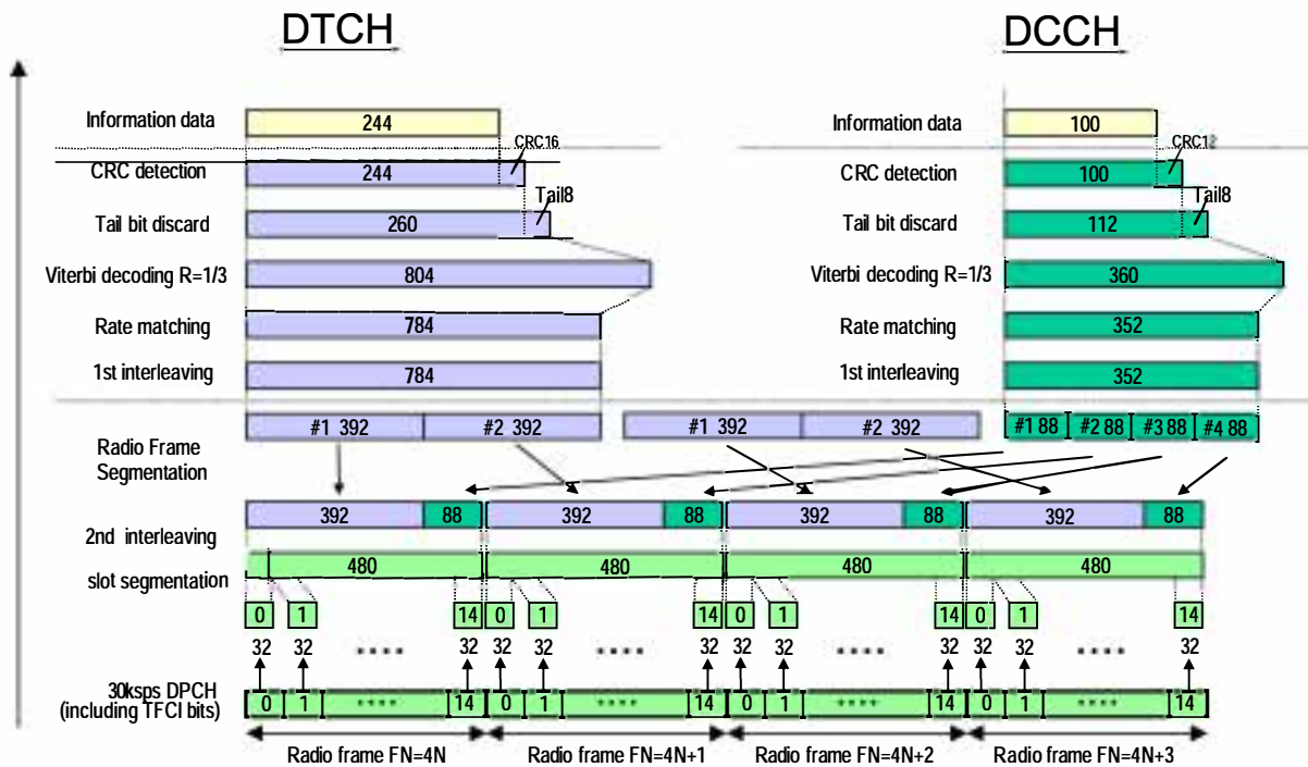
Figure A.11A (Informative): Channel coding of DL reference measurement channel for requirements using DPCCCH with 4 channel bits (12.2 kbps)
