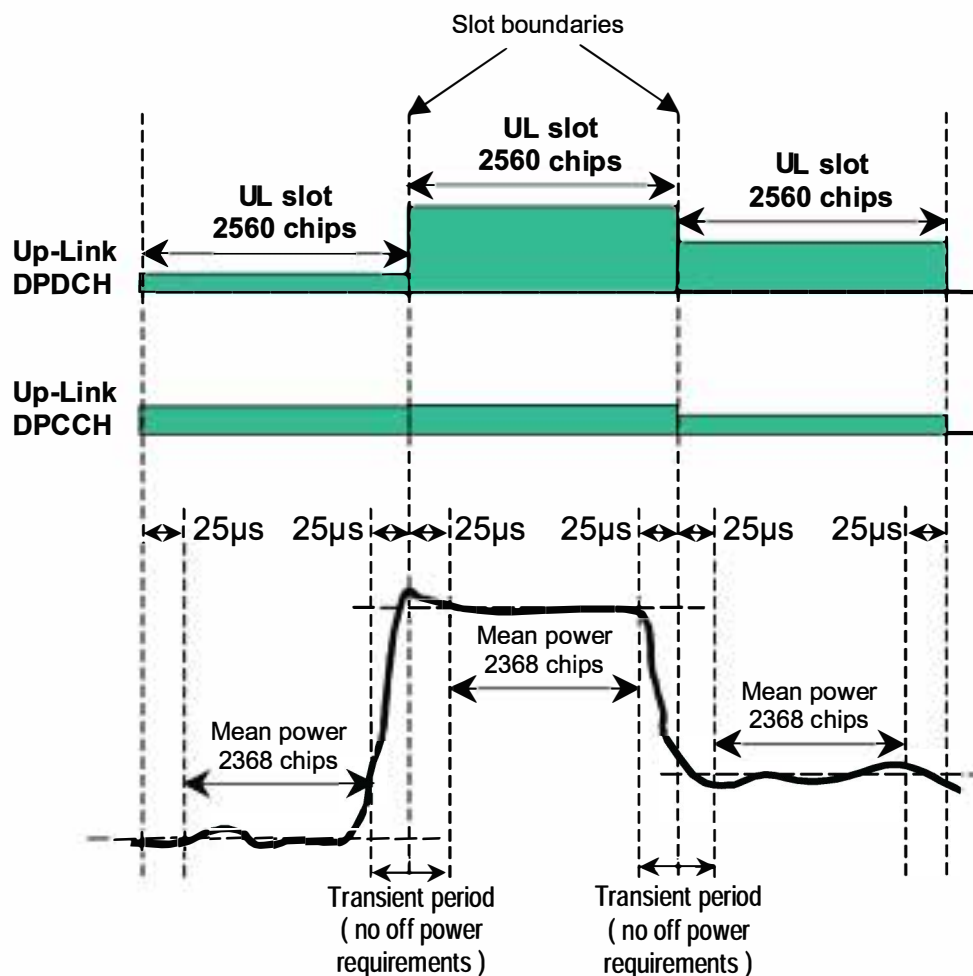
Figure 6.4: Transmit template during TFC change
