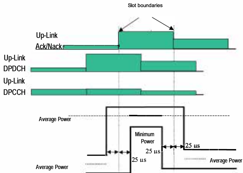
Figure 6.5A: Transmit template during Ack/Nack transmission
