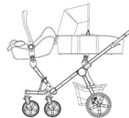
Reference drawing illustrating the status of usage of the present invention additionally installed with a storage basket + a safety seat + a hand held sleeping basket
