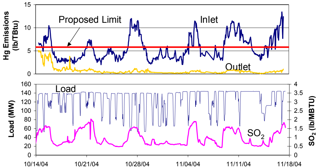
Figure 2. Mercury and SO 2 Trends during Long-Term Testing.
