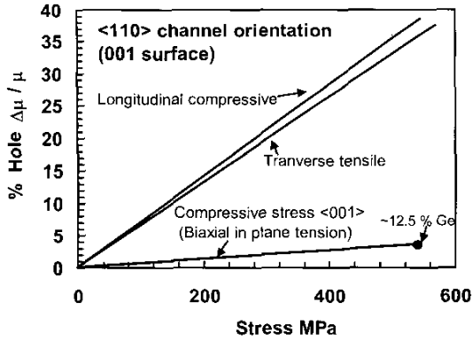
Fig. 1 Hole mobility gain vs. stress from the piezo coefficients in [3].
