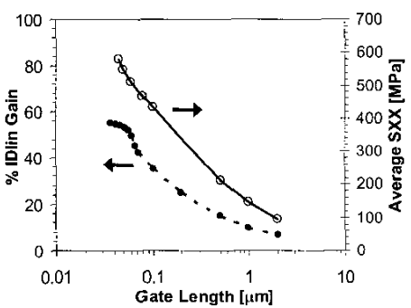
Fig. 8 Avg. PMOS channel stress (SXX) and % I_{\text{DLIN}} gain [corrected for (V_G-V_T) ] vs. L_{\text{GATE}}
