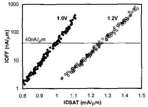
Fig. 5 NMOS Ion/Ioff curve at 1.2V & 1.0V. At 1.0V & I_{\text{OFF}}=40\text{nA}/\mu\text{m} , I_{\text{DSAT}}=1.01\text{mA}/\mu\text{m}
