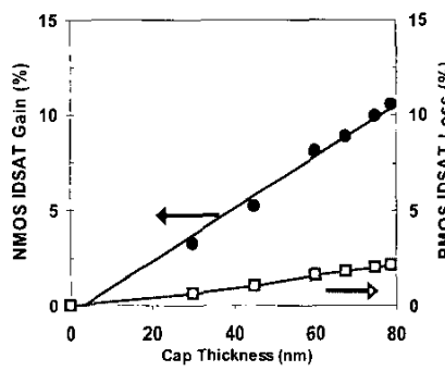
Fig. 7 N & P I_{\text{DSAT}} vs. nitride capping layer thickness.
