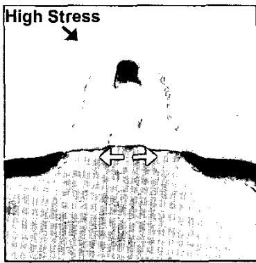
Fig. 3 TEM of NMOS transistor showing high tensile stress nitride overlayer.
