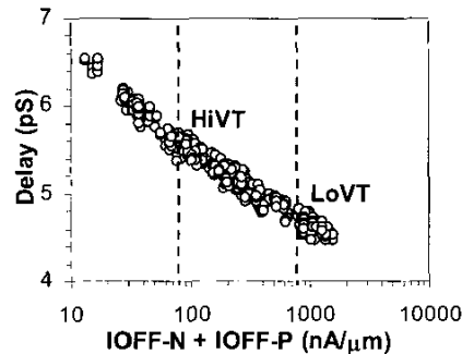
Fig. 10 Ring Oscillator delay for fanout=1 vs. sum of NMOS and PMOS I_{\text{OFF}} .
