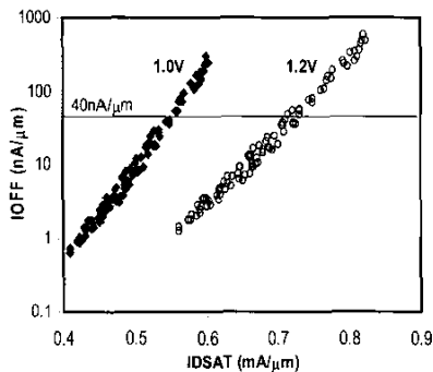
Fig. 6 PMOS Ion-Ioff at 1.2V & 1.0V. At 1.0V & I_{\text{OFF}}=40\text{nA}/\mu\text{m} , I_{\text{DSAT}}=0.55\text{mA}/\mu\text{m} .
