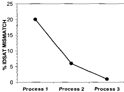
Fig. 9 PMOS I_{\text{DSAT}} mismatch for minimum pitch vs. 1.5X min pitch.
