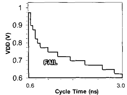
Fig. 11 Schmoos of 50Mb SRAM operating down to V_{\text{DD}}=0.65\text{V} .
