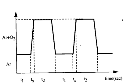
a) Fig. 1 Reactive dc magnetron sputtering process; a) Schematic diagram of process ( t_1 period = Ar ambient, t_2 = Ar+O 2 ambient, t_s = O 2 flow stabilization period), b) Film thickness is linearly proportional to the process cycles.
