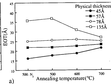
Fig. 7 The effect of annealing in oxygen ambient on a) EOT and b) Leakage current at V_g=+1V .
