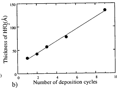
a) Fig. 1 Reactive dc magnetron sputtering process; a) Schematic diagram of process ( t_1 period = Ar ambient, t_2 = Ar+O 2 ambient, t_s = O 2 flow stabilization period), b) Film thickness is linearly proportional to the process cycles.
