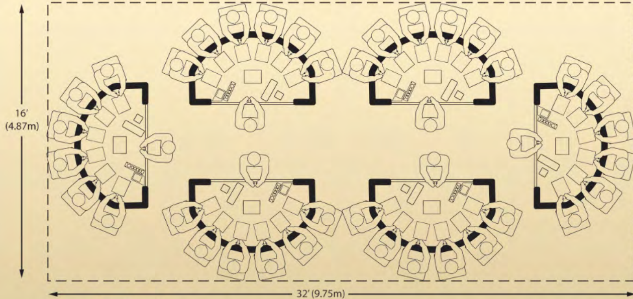
DTS-V Pit dimensions and recommended space requirements for a 6 table pit.
