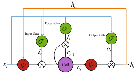
Fig. 3. LSTM model
