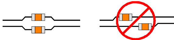
Fig. 9. Lumping discontinuities
