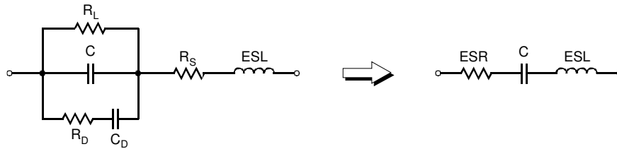
Fig. 16. Capacitor losses modeled by a series resonance circuit
