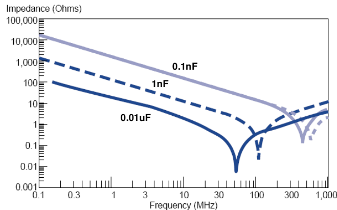
Fig. 17. Capacitor impedance versus frequency
