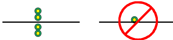
Fig. 10. Avoiding via clearance sections
