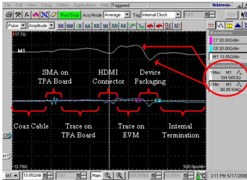
Fig. 6. TDR display revealing the locations of discontinuities
