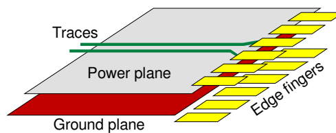
Fig. 11. Keeping planes out of the area between edge-fingers
