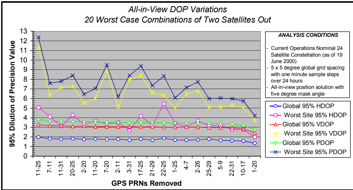
Figure A-3-3. Worst-Case DOP Values with Two Satellites Out
