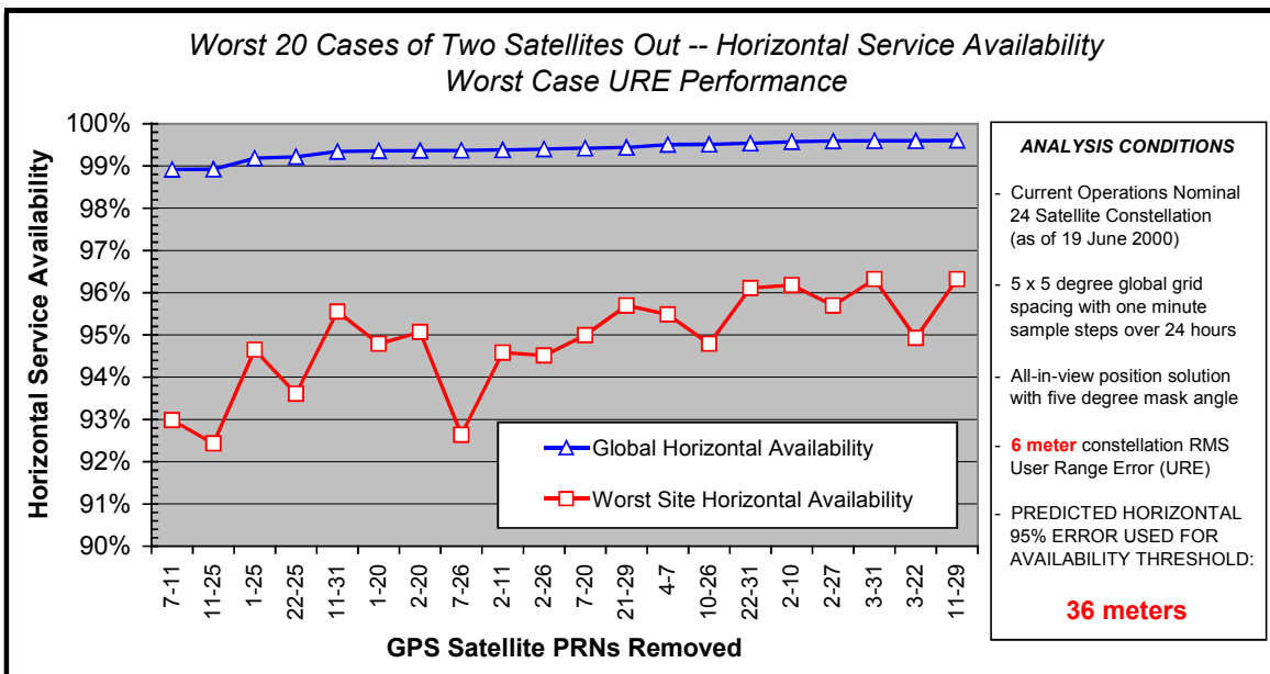
Figure A-3-4. GPS Horizontal Availability – Two Satellites Out
