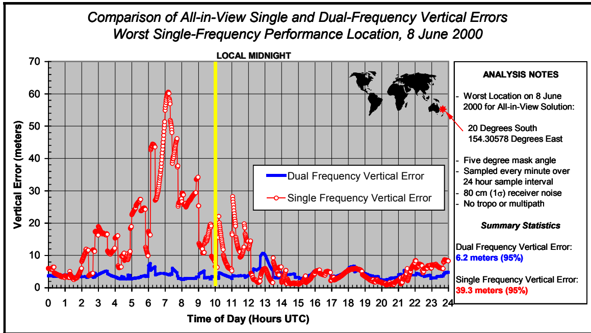
Figure A-5-18. Example Worst Site Single-Frequency Vertical Performance
