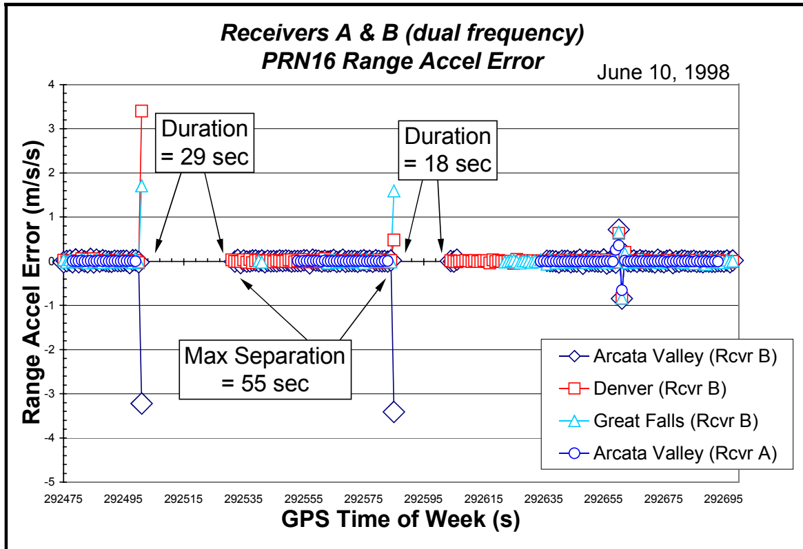
Figure A-4-1. Dual-Frequency Receiver Response (PRN 16 Anomaly)
