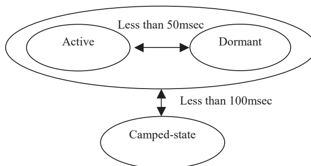
Figure 6.1 an example of state transition
