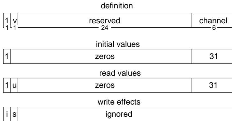
Figure 8-14A — BROADCAST_CHANNEL format
