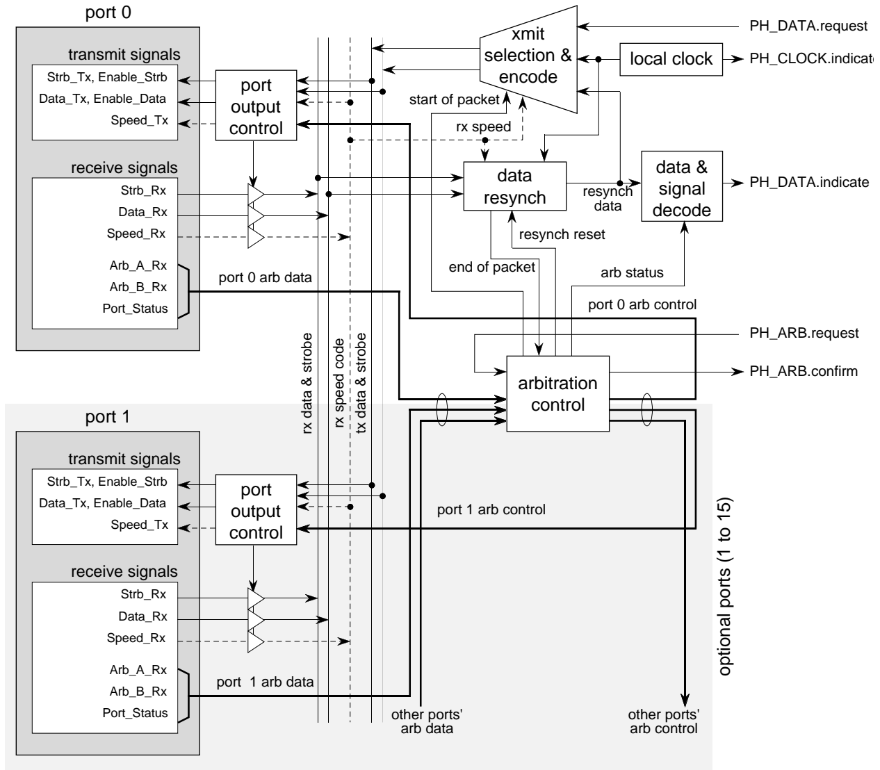
Figure 4-21 — Cable physical layer architecture
