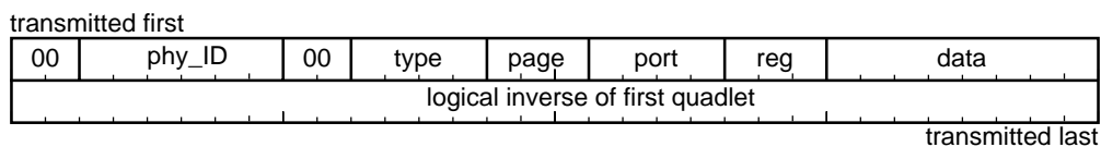
Figure 4-20C—Remote reply packet format
