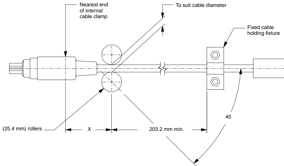
Figure 4-11M — Fixture for cable flex test
