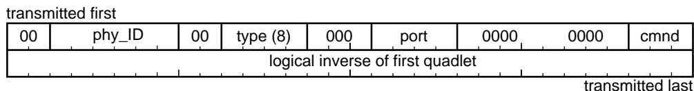
Figure 4-20D — Remote command packet format
