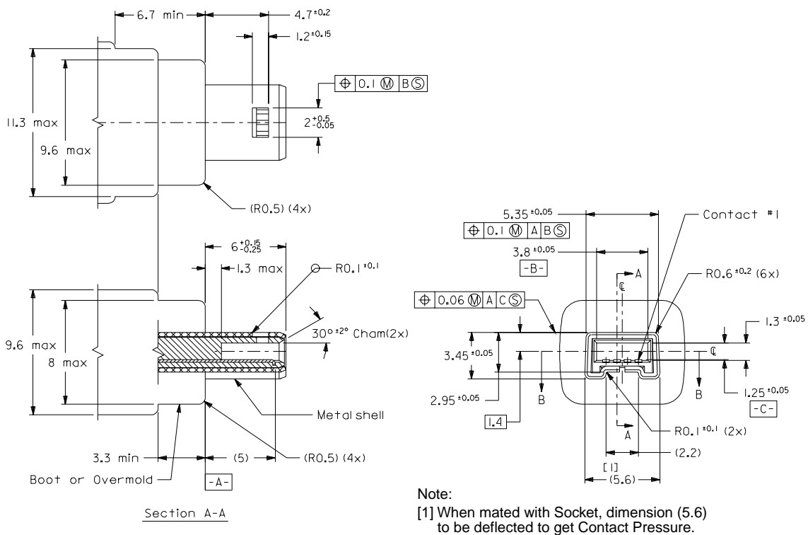
Figure 4-11A — Plug body
