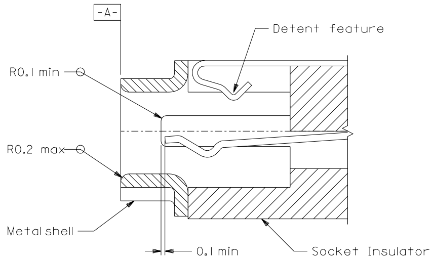
Figure 4-11D — Socket cross-section A-A
