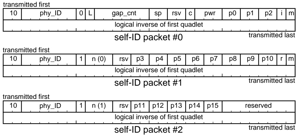
Figure 4-18—Self-ID packet formats
