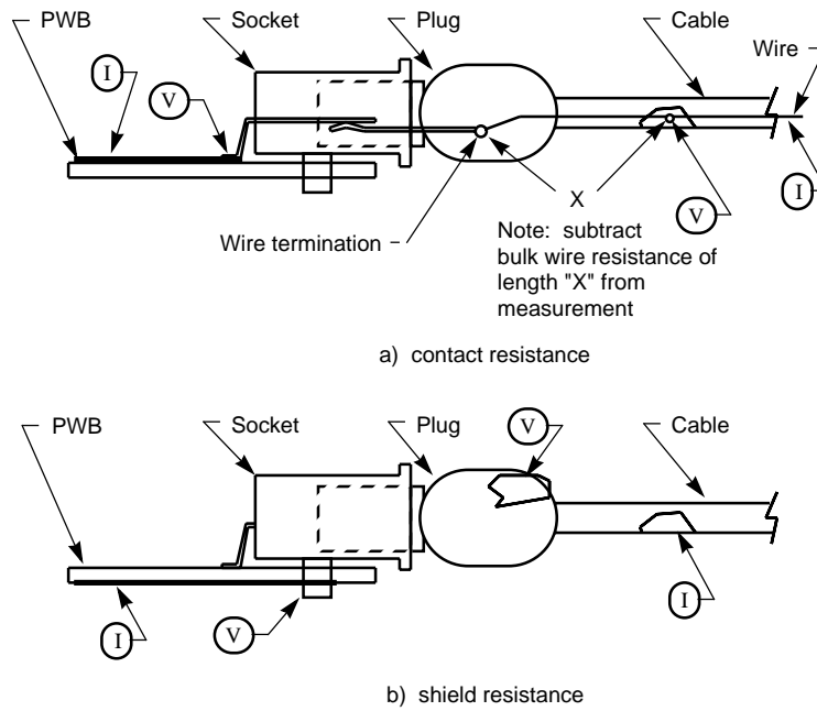
Figure 4-11L — Shield and contact resistance measuring points
