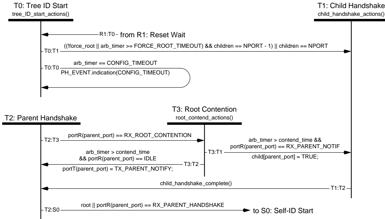
Figure 4-23 — Tree ID state machine
