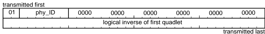
Figure 4-19—Link-on packet format
