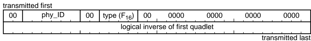
Figure 4-20F — Resume packet format
