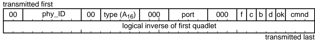
Figure 4-20E — Remote confirmation packet format
