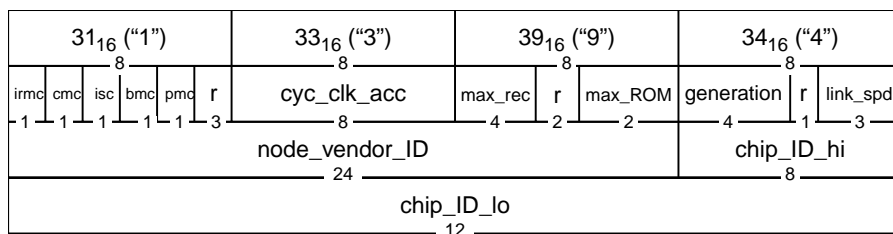
Figure 8-20 — Bus_Info_Block format
