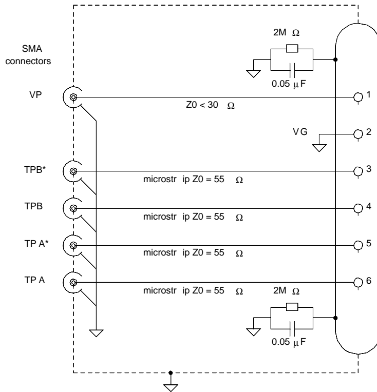
Figure K-3A — Differential test fixture schematic
