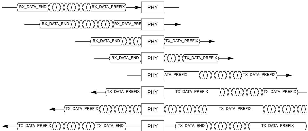
Figure 3-32 — Fly-by concatenation
