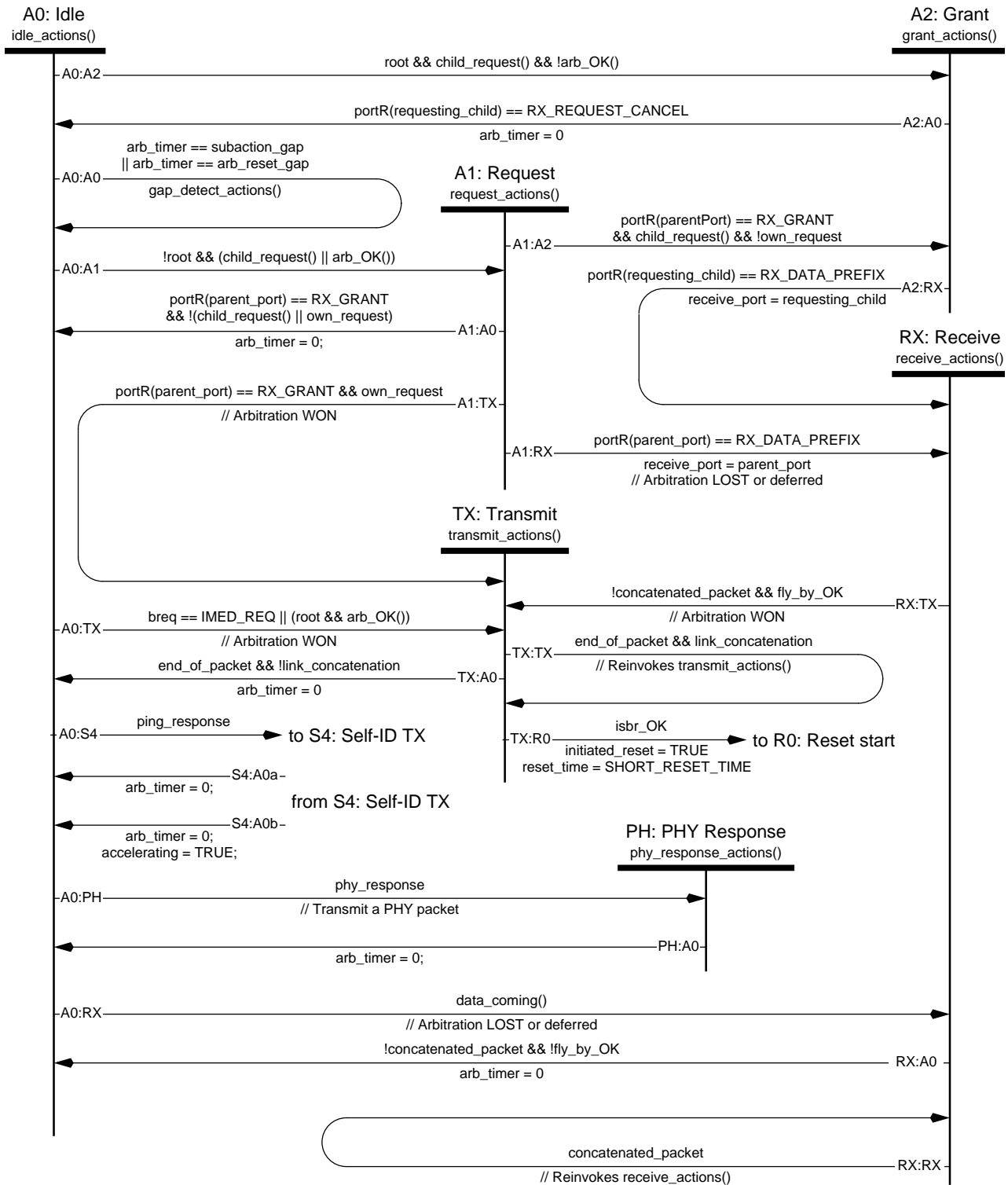
Figure 4-25 — Cable arbitration state machine
