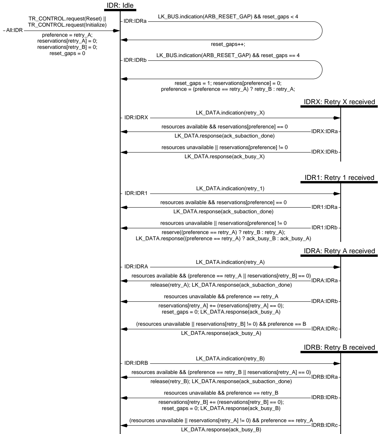
Figure 7-3—Inbound subaction dual-phase retry state machine
