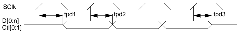
Figure 5A-13 — PHY to link transfer waveform at the PHY
