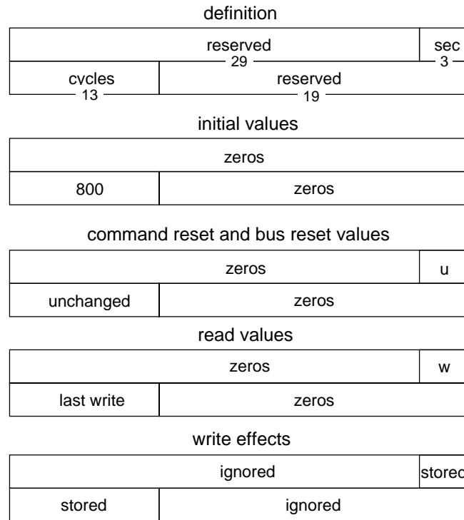
Figure 8-4 — SPLIT_TIMEOUT format
