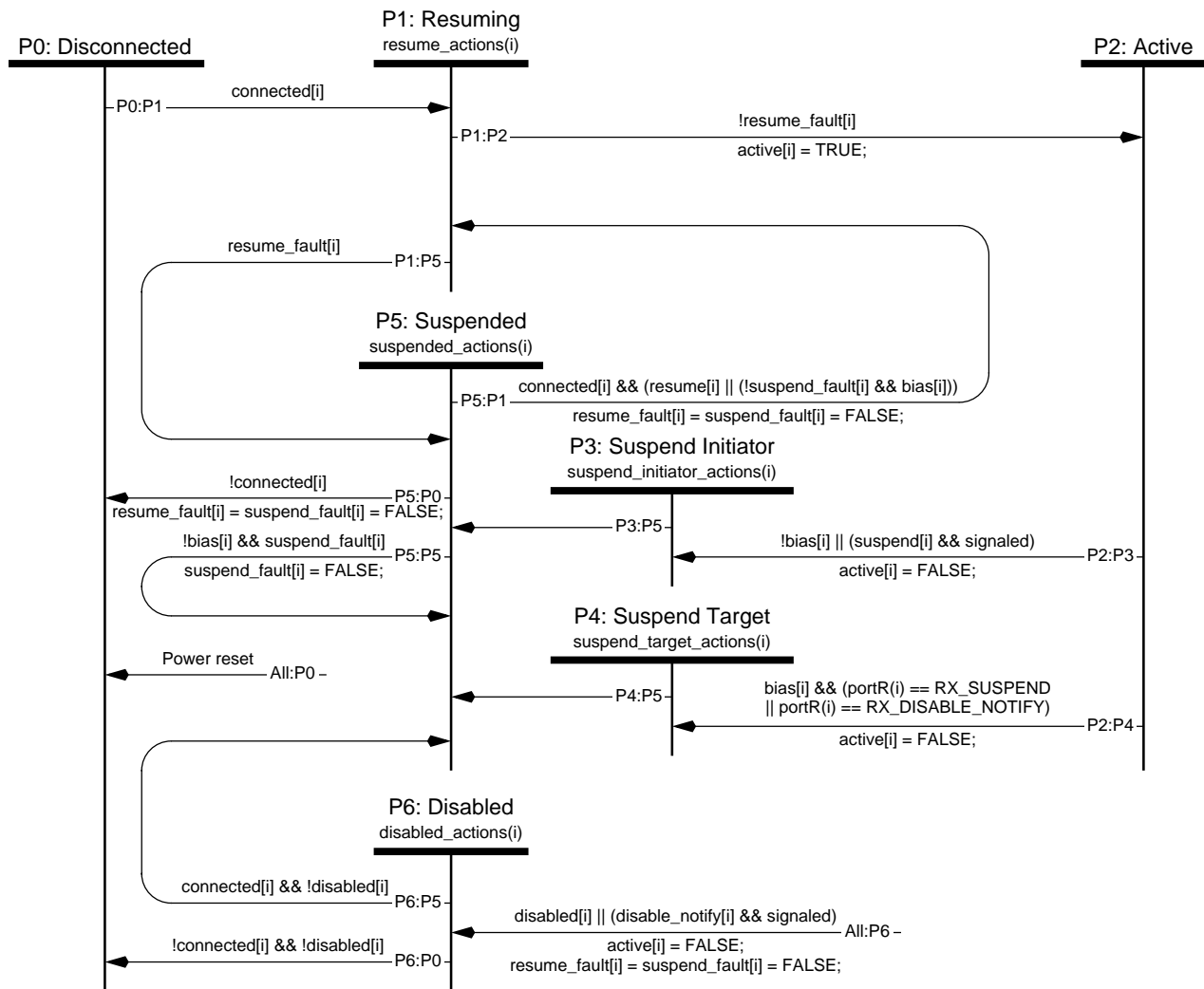
Figure 4-26 — Port connection state machine
