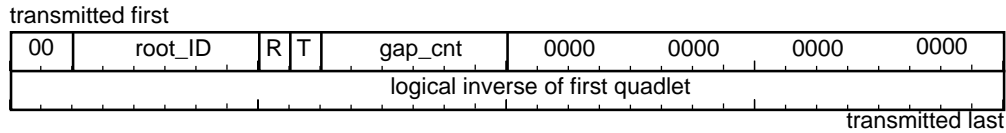
Figure 4-20—PHY configuration packet format
