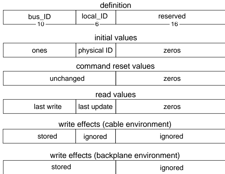
Figure 8-3 — NODE_IDS format
