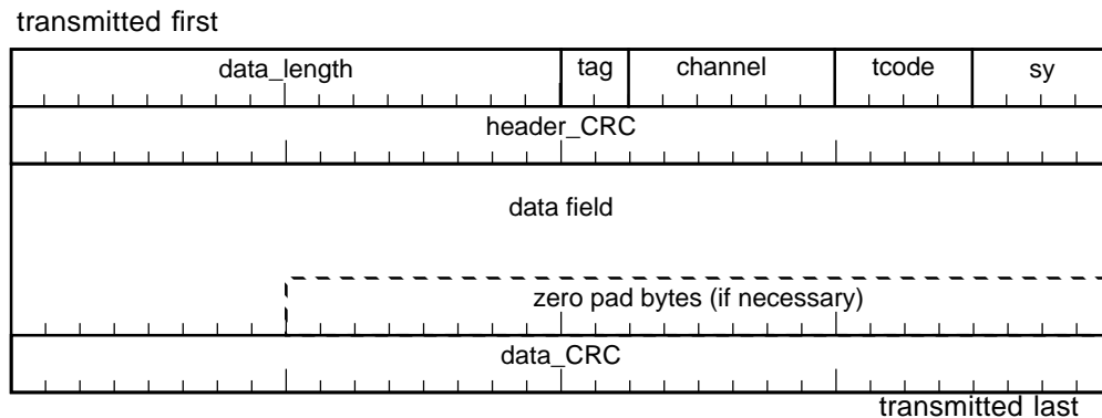
Figure 6-17A — Asynchronous stream packet format
