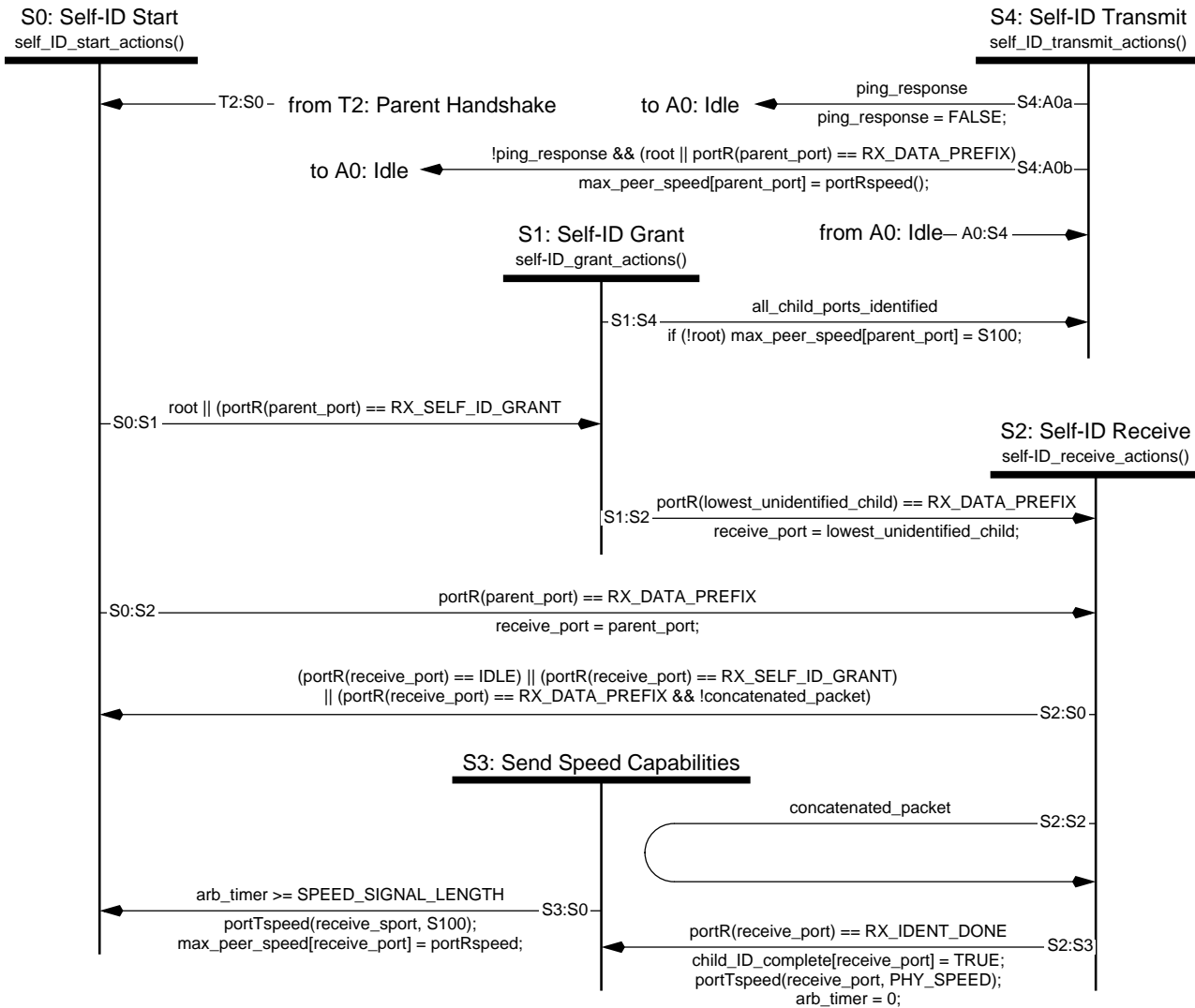
Figure 4-24 — Self-ID state machine
