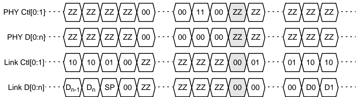
Figure 5A-8 — Transmit timing
