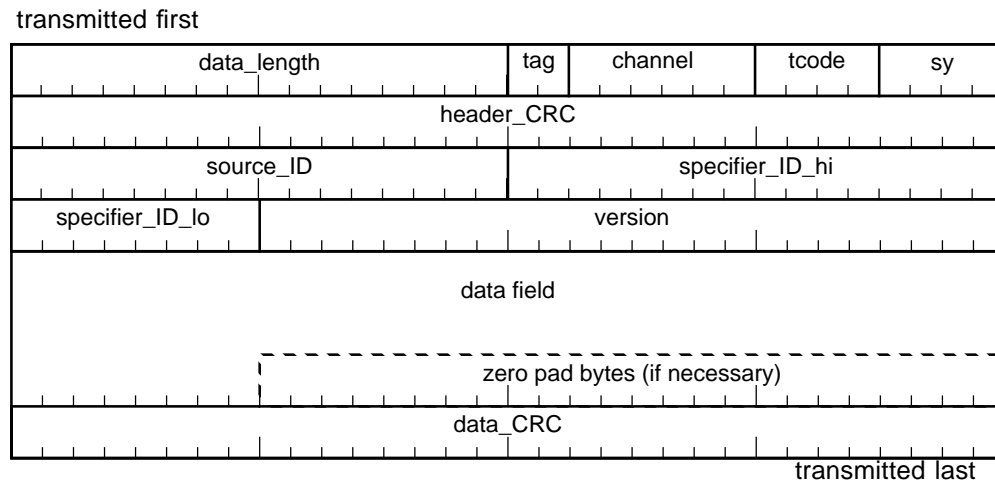
Figure 6-17B — Global asynchronous stream packet (GASP) format
