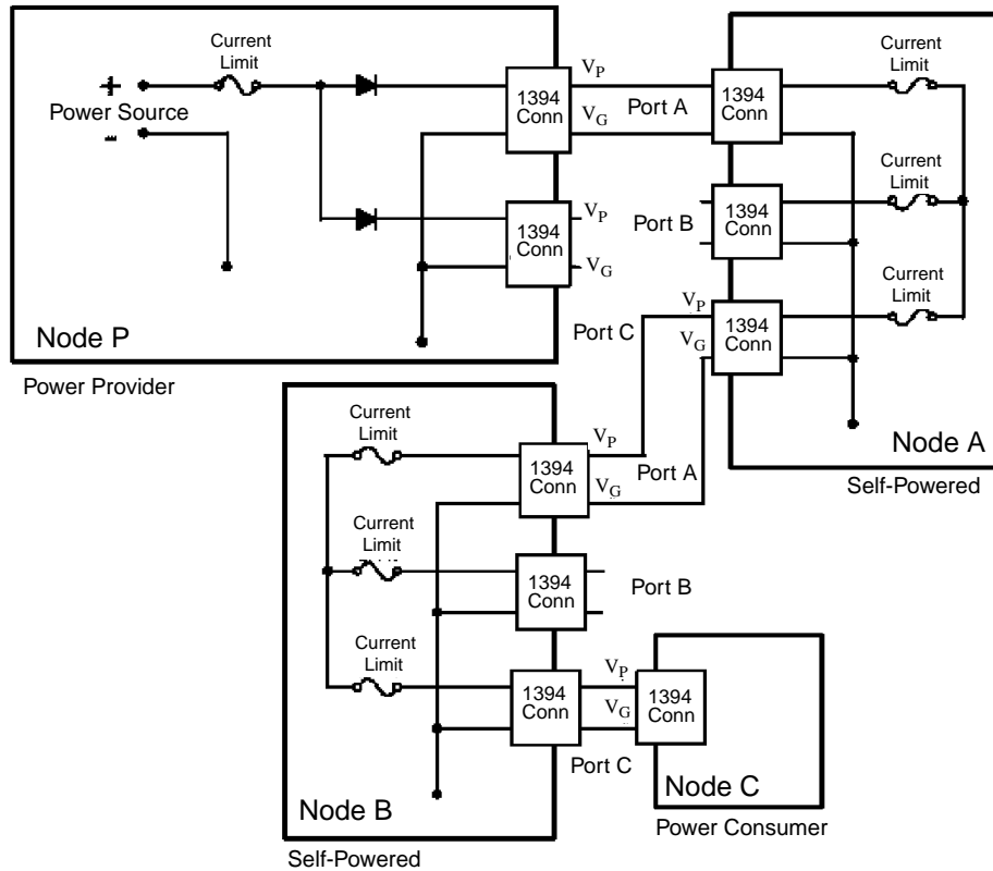
Figure M-1 — Power distribution example
