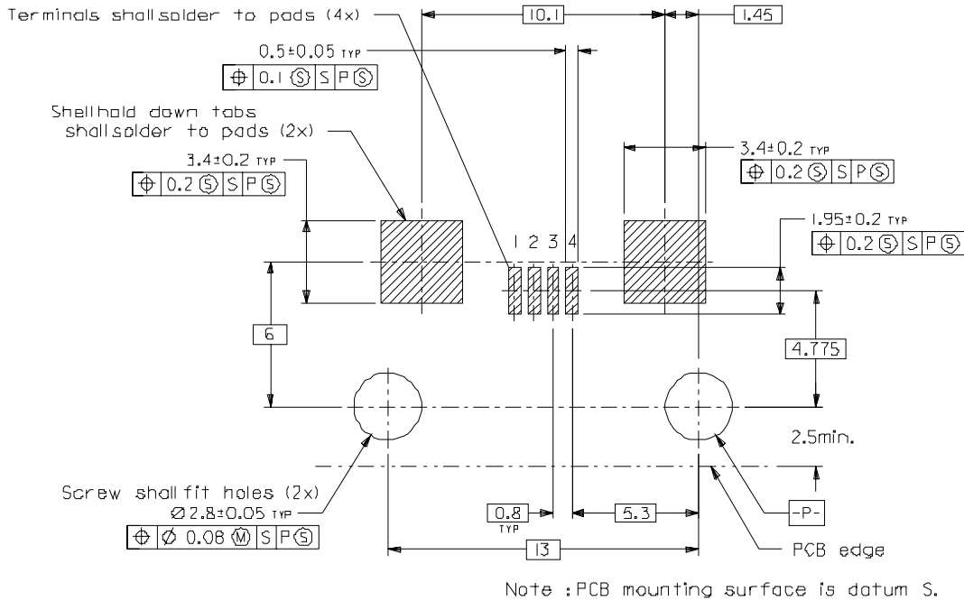
Figure 4-11G — Flat surface-mount printed circuit board socket footprint
