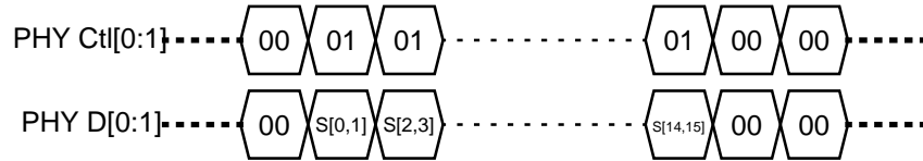
Figure 5A-7 — Status timing
