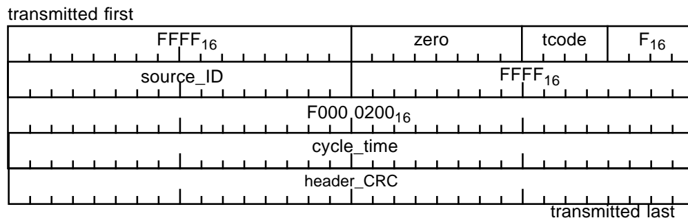
Figure 6-10 — Cycle start packet format
