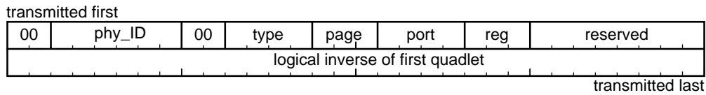
Figure 4-20B—Remote access packet format
