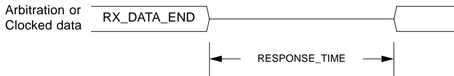
Figure 4-20J — Subaction response
