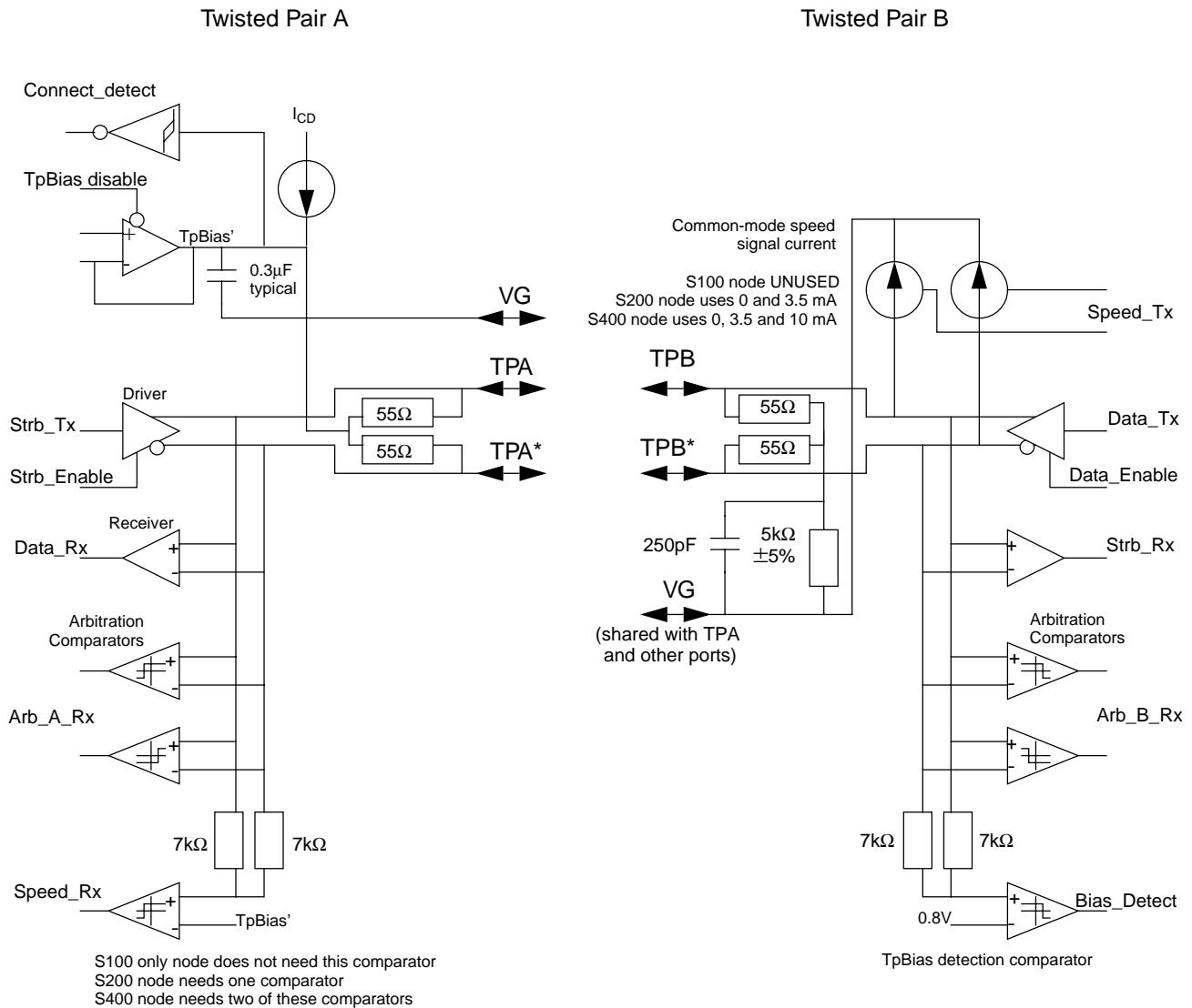
Figure 4-12 — Port interface
