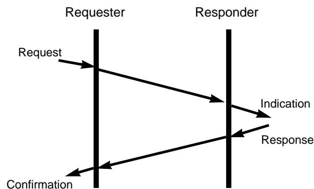
Figure 1-2—Service model
