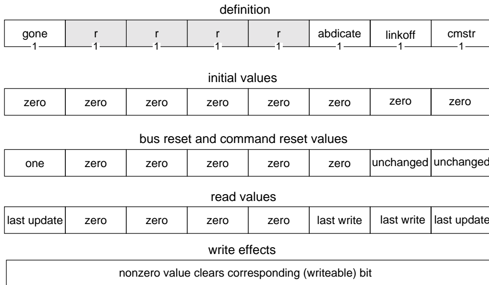
Figure 8-2 — STATE_CLEAR.bus_depend field
