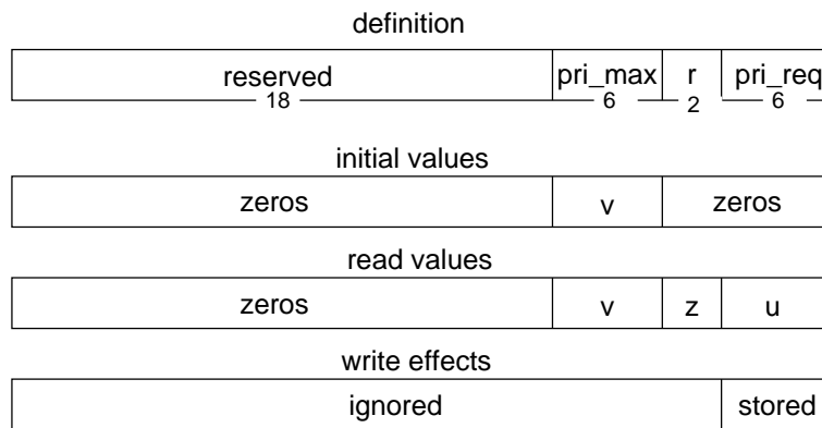
Figure 8-9A—PRIORITY_BUDGET format
