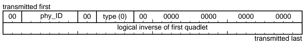
Figure 4-20A—Ping packet format
