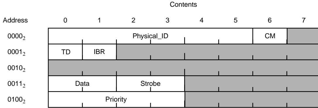
Figure 5B-4 — PHY register map for the backplane environment
