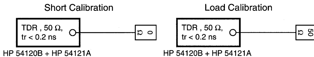
Figure K-4—Signal pairs impedance setup calibration
