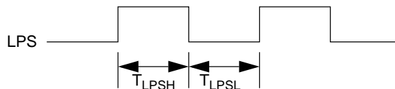
Figure 5A-3 — LPS waveform when differentiated
