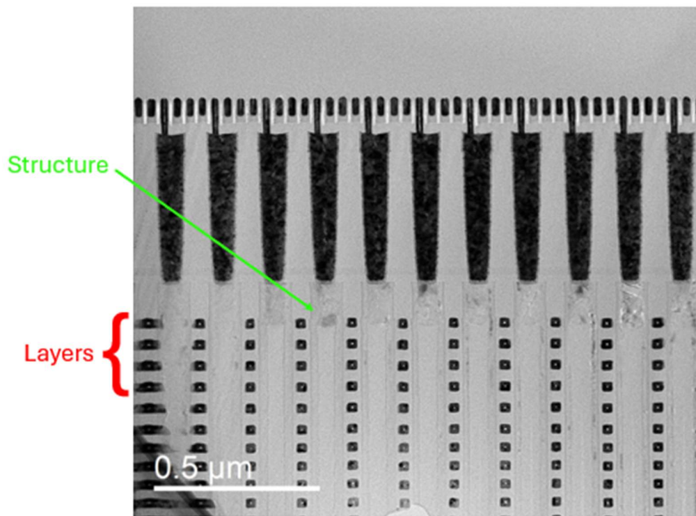
Figure 1 - TEM Image of Micron 7450
