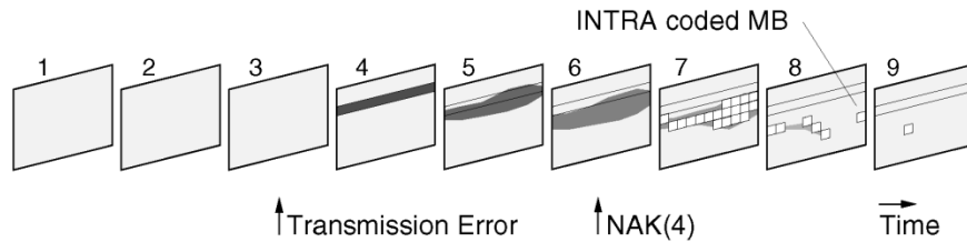
Fig. 5. Illustration of error propagation when error tracking is used.
