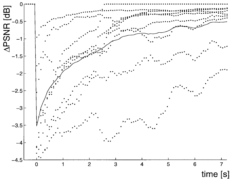
Fig. 3. Loss in SNR of the decoded video signal after previous frame concealment of one GOB.
