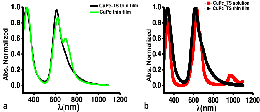
Figure 5.26 Absorption peaks for a) standard CuPc and CuPc_TS b) CuPc_TS in solution and solid states.
