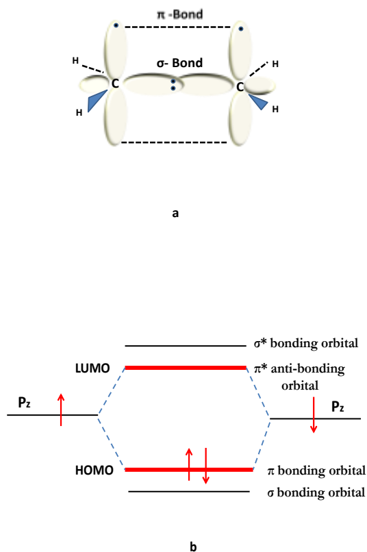
Figure 2.8 a) sp^2 hybridization in ethylene. b) Energy level splitting in the hybridized sp^2 states.
