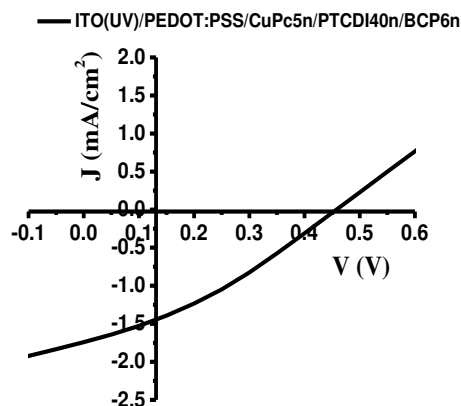
Figure 6.2 J-V characteristic for the cell consists of ITO/PEDOT:PSS/CuPc5nm/PTCDI40nm/BCP6nm.
