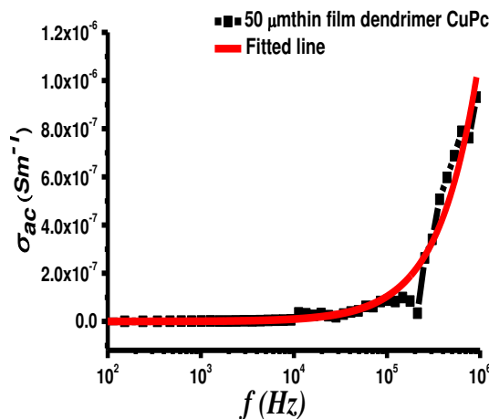
Figure 5.15 Dendrimer CuPc thin film conductivity as a function of frequency under room temperature and humidity ( \sim 20\% RH).
