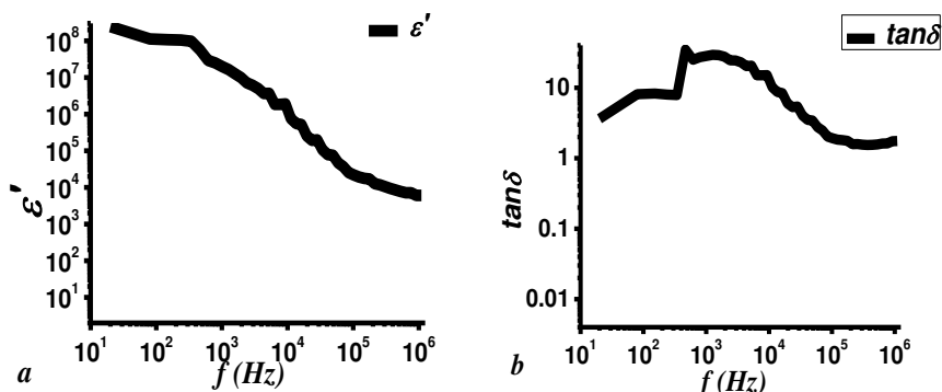
Figure 5.27 Polyaniline salt pellets a) dielectric constant b) tangent loss factor.
