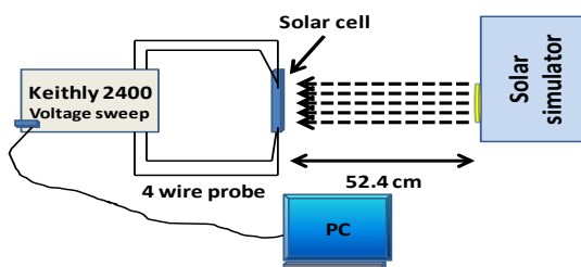
Figure 4.6 J-V characterization set up, a voltage seep is applied by Keithly 2400, the V_{oc} , J_{sc} , FF and \eta are extracted by the PC software.
