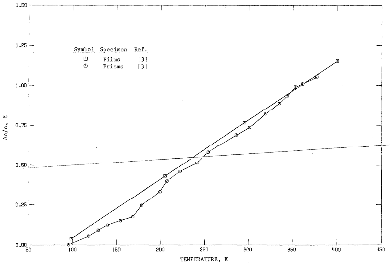
FIGURE 6. VARIATION OF REFRACTIVE INDEX OF SILICON WITH TEMPERATURE AT WAVELENGTH 3 μm [3]
