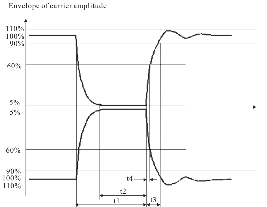
Figure 1 – Pulse shape
