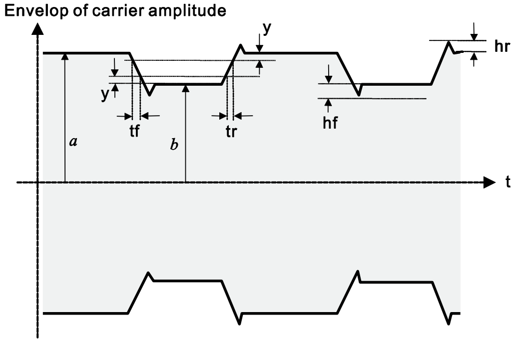
Figure 2 — Modulated Waveform
