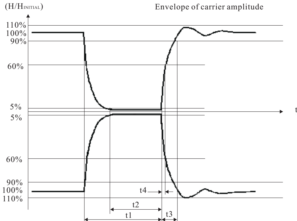
Figure 1 — Pulse shape
