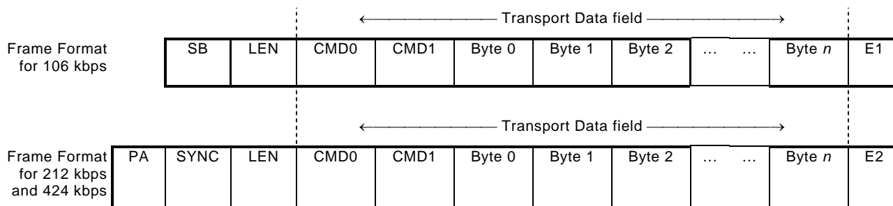
Figure 23 — Transport Frame format Definition
