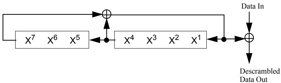
Figure 113—Data scrambler
