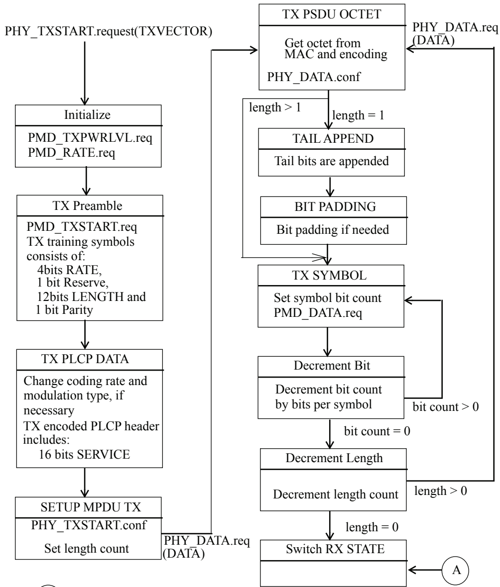
Figure 123—PLCP transmit state machine
