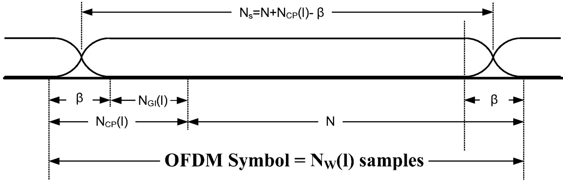
1765 Figure 7-20/G.9960 – Structure of an OFDM symbol with cyclic extension and overlapped 1766 windowing
