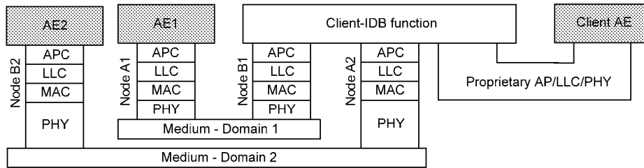
Figure 5-10/G.9960 – Protocol stack of inter-domain communication
