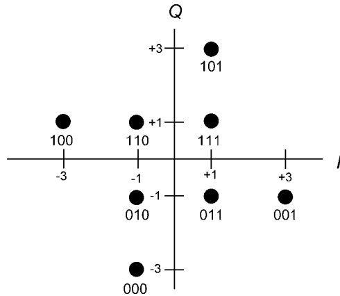
Figure 7-16/G.9960 - Constellation and mapping for b = 3
