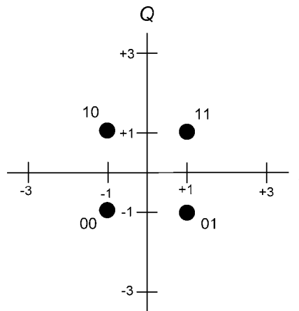
Figure 7-13/G.9960 - Constellation and mapping for b = 2
