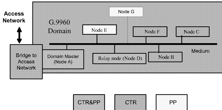
Figure II-2/G.9960 – Example of HN containing single domain using UM (combined PP& CTR)
