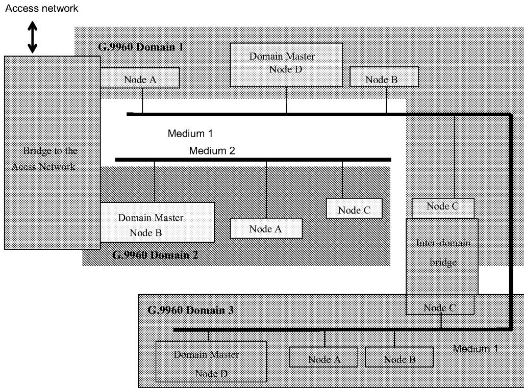
Figure II-3/G.9960 – Example of HN comprising three domains
