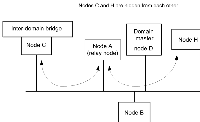
479 Figure 5-4/G.9960 – A domain operating in Unified mode (UM) containing hidden nodes
