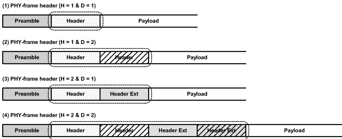
Figure 1: Header repetition scheme (D, H = 1 or 2)
