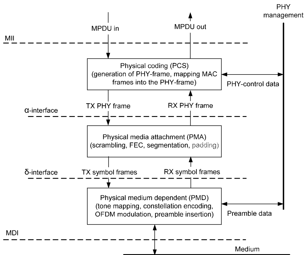
853 Figure 7-1/G.9960 – Functional model of the PHY
