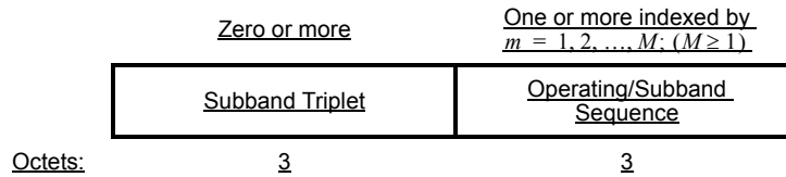
Figure 8-90c—Triplet field if dot11OperatingClassRequired is true
