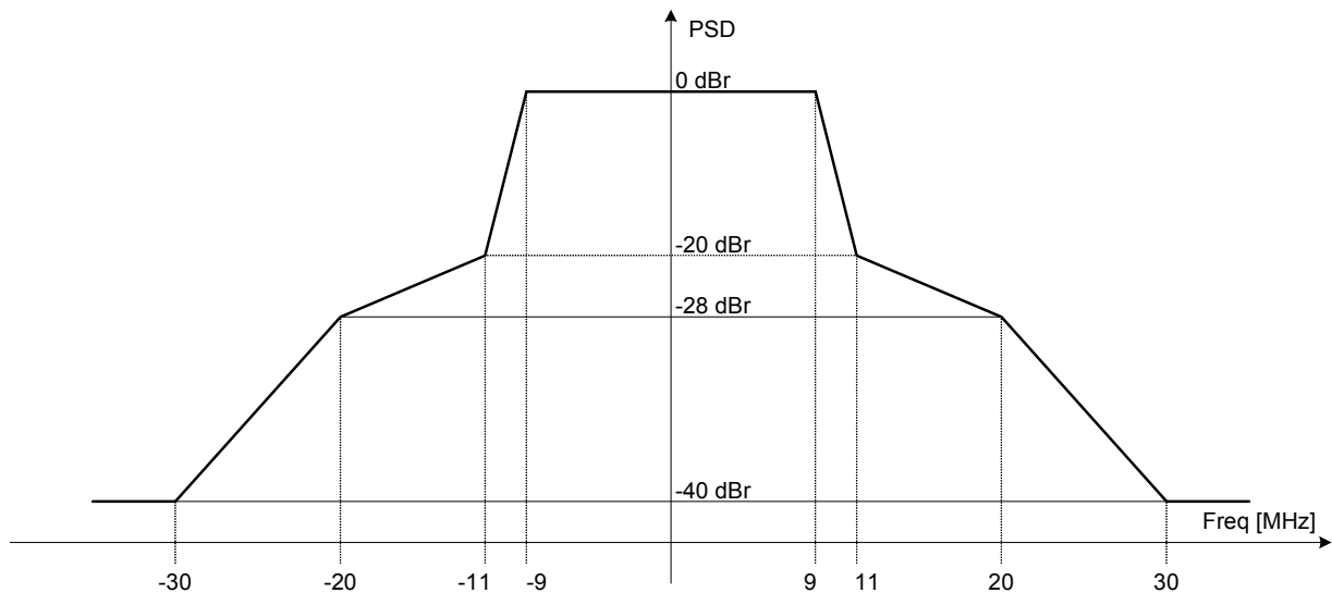
Figure 22-29—Example transmit spectral mask for a 20 MHz mask PDU
