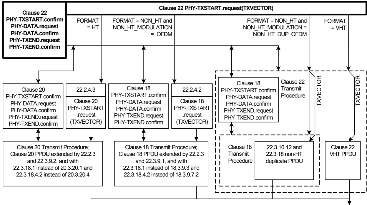
Figure 22-1— PHY interaction on transmit for various PDU formats
