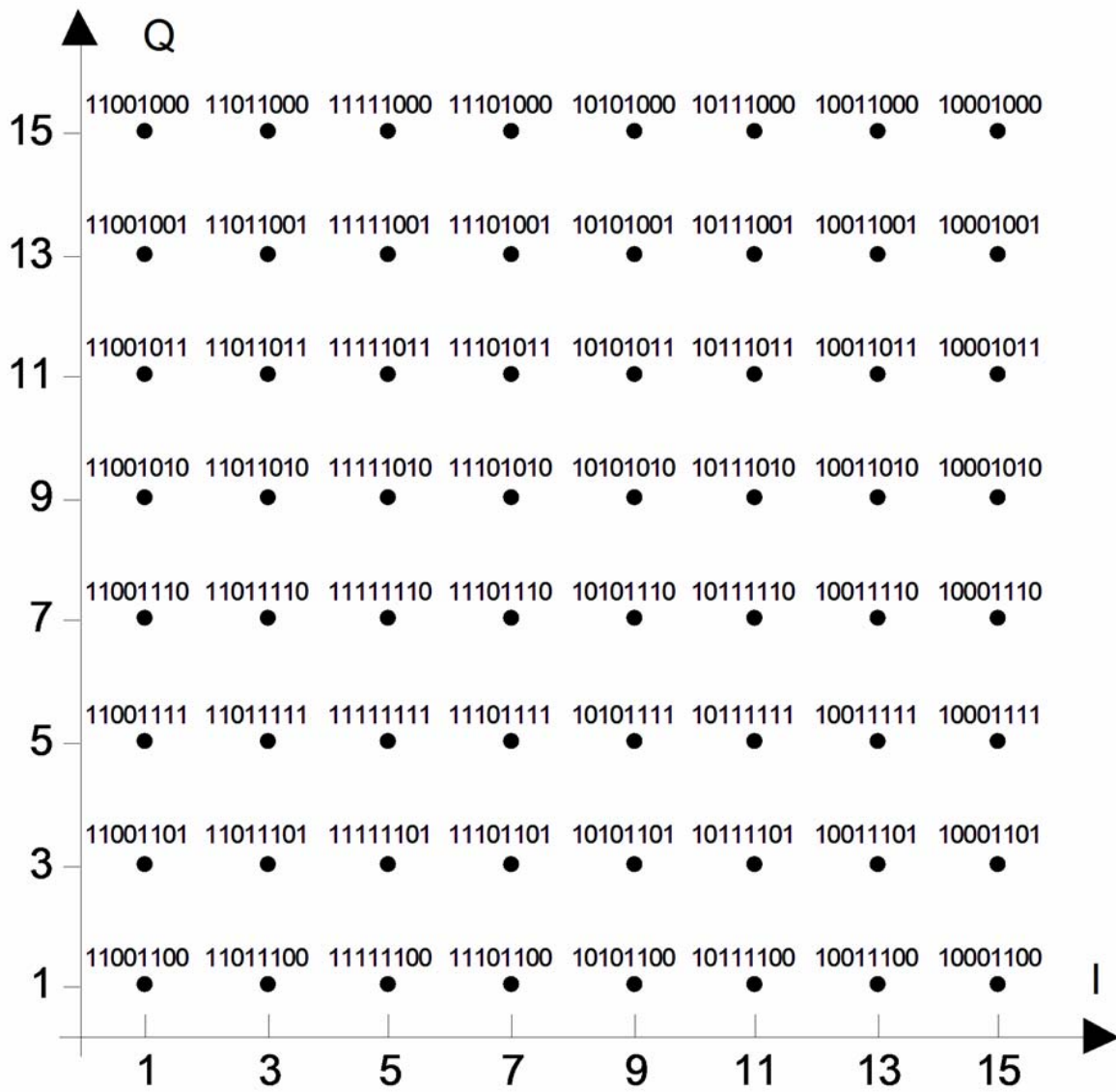
Figure 22-24—Constellation bit encoding for 256-QAM (1st quadrant)
