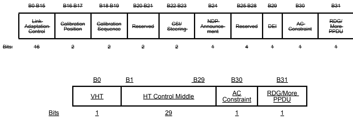
Figure 8-5—HT Control field
