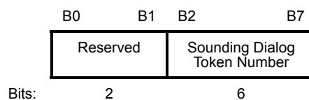
Figure 8-29k—Sounding Dialog Token field
