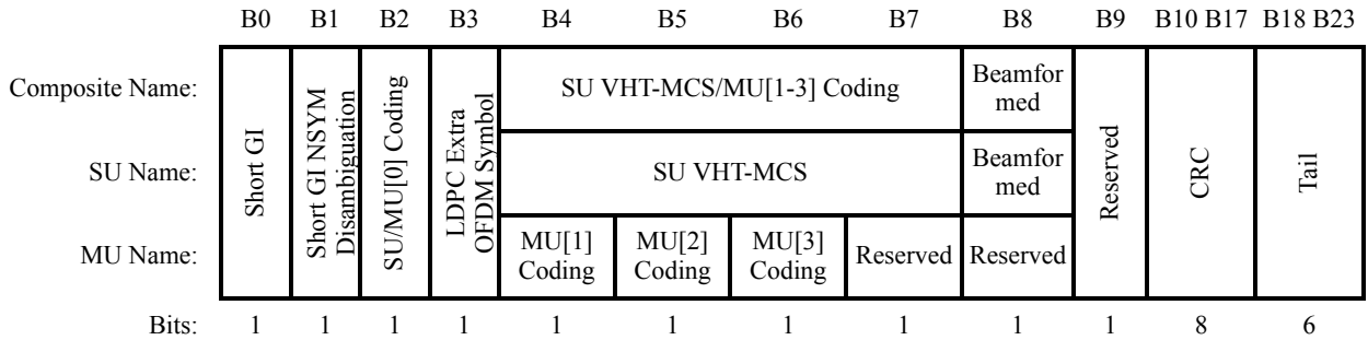
Figure 22-19—VHT-SIG-A2 structure
