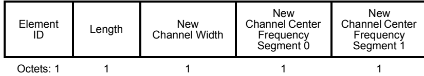
Figure 8-401bw—Wide Bandwidth Channel Switch element format
