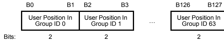
Figure 8-80g—User Position Array field
