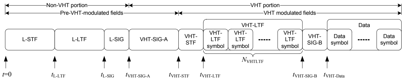
Figure 22-17—Timing boundaries for VHT PPDU fields
