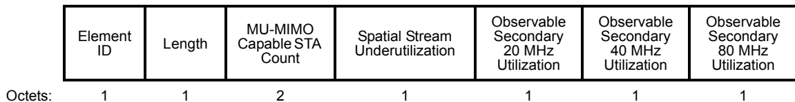
Figure 8-401bv—Extended BSS Load element format
