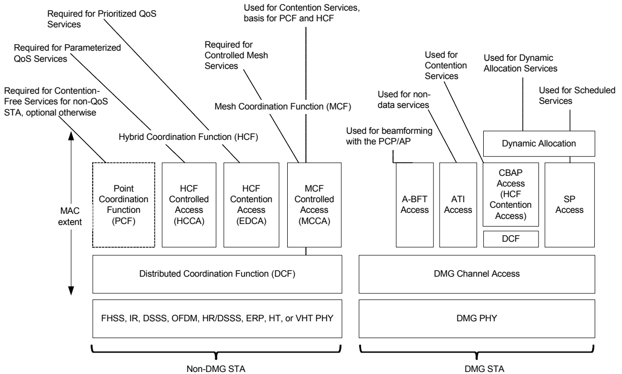
Figure 9-1—MAC architecture
