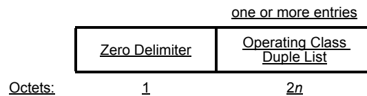
Figure 8-246b—Operating Class Duple Sequence field format
