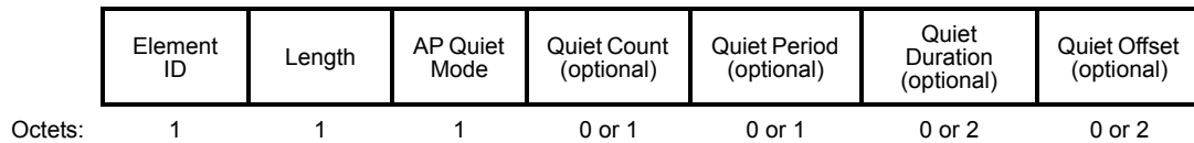
Figure 8-401cb—Quiet Channel element format
