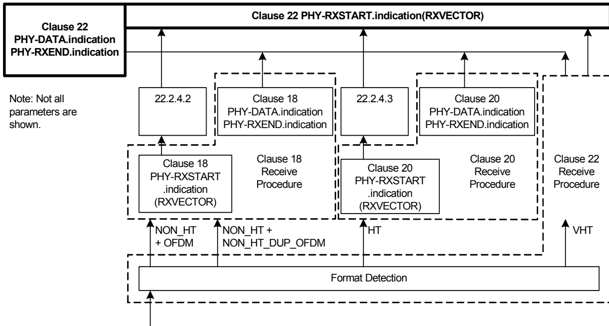
Figure 22-2—PHY interaction on receive for various PPDU formats
