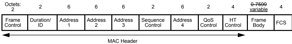
Figure 8-30—Data frame
