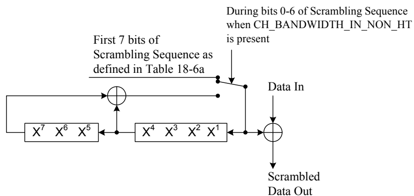
Figure 18-7—Data scrambler
