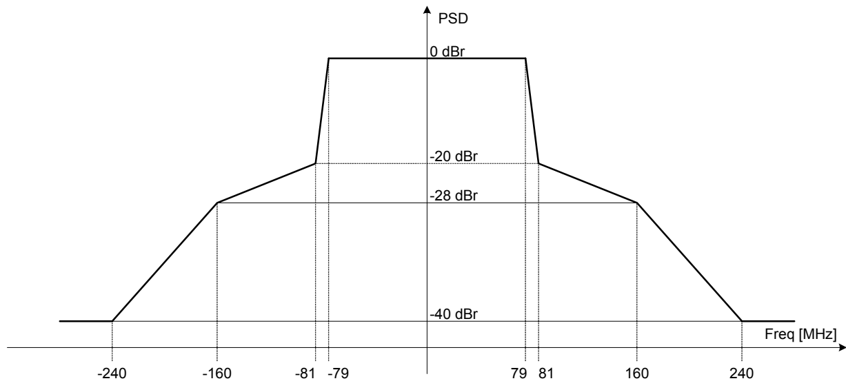
Figure 22-32—Example transmit spectral mask for a 160 MHz mask PDU
