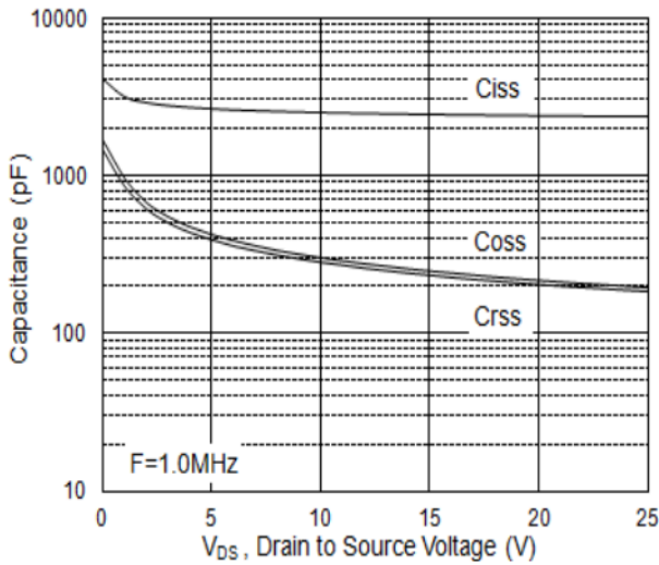
Fig. 9: Capacitance
