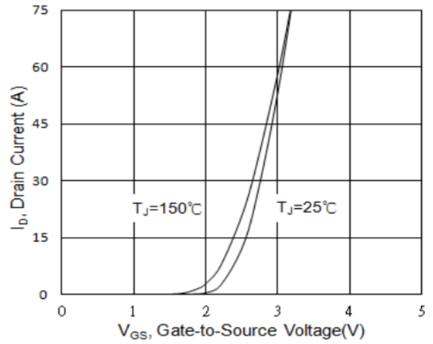
Fig. 8: Transfer Characteristics
