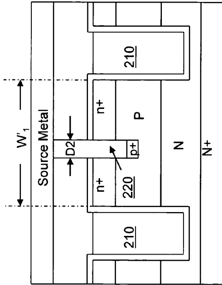
Fig. 3B (E-E' Cross Section)
