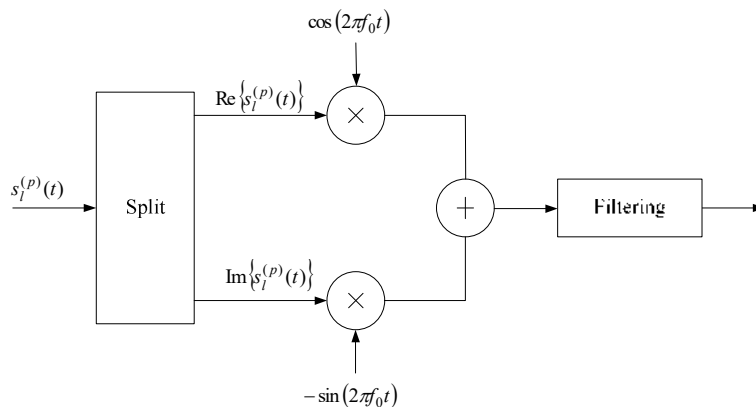
Figure 6.13-1: Downlink modulation
