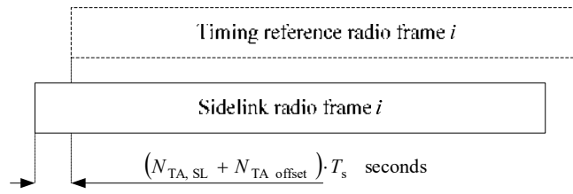
Figure 9.9-1: Sidelink timing relation.
