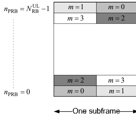
Figure 5.4.3-1: Mapping to physical resource blocks for PUCCH formats 1 – 3
