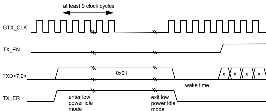
Figure 35-8—LPI transition
