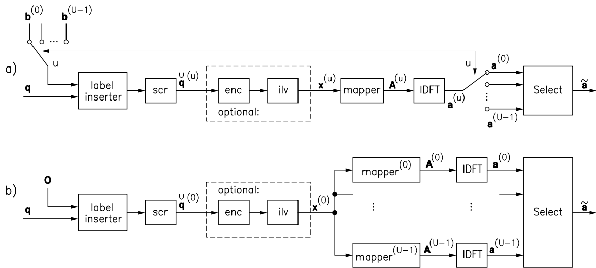
Fig. 1. OFDM transmitter incorporating the extended SLM scheme with a scrambler.
