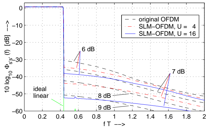
Fig. 7. Comparison of the power spectral density of s'(t) at the output of the power amplifier (modelled by a soft-limiter) between OFDM without and with the extended SLM scheme with different numbers of generated candidate sequences and for various backoffs.
