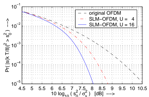
Fig. 5. Probability that the instantaneous power of the transmit signal s(t) exceeds the value s_0^2 .
