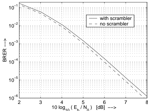
Fig. 6. Bit residual error rate after decoding without and with the scrambling SLM scheme.
