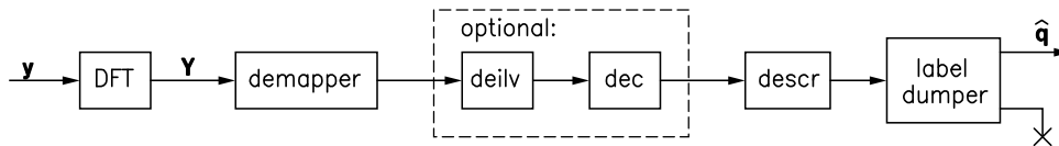
Fig. 3. Corresponding OFDM receiver for the extended SLM scheme.
