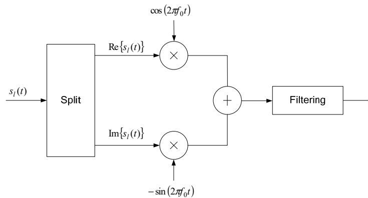
Figure 5.8-1: Uplink modulation.
