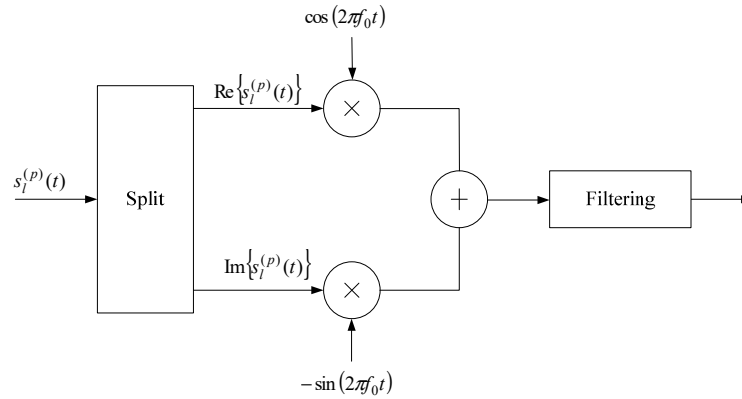
Figure 6.13-1: Downlink modulation.
