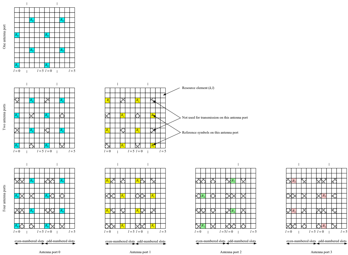
Figure 6.10.1-2. Mapping of downlink reference signals (extended cyclic prefix).
