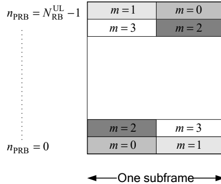
Figure 5.4.3-1: Mapping to physical resource blocks for PUCCH.
