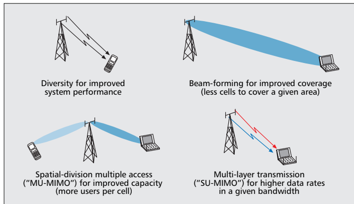
■ Figure 5. Multiple-antenna techniques in LTE.
