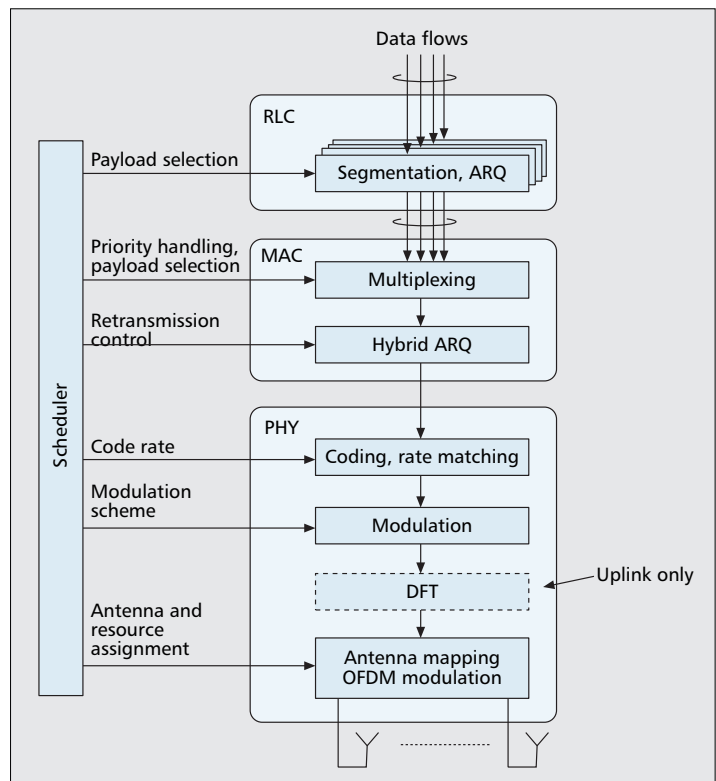
■ Figure 1. LTE protocol structure (simplified).
