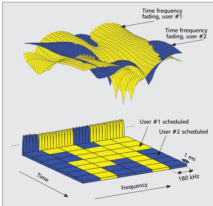
■ Figure 3. Channel-quality variations in frequency and time.
