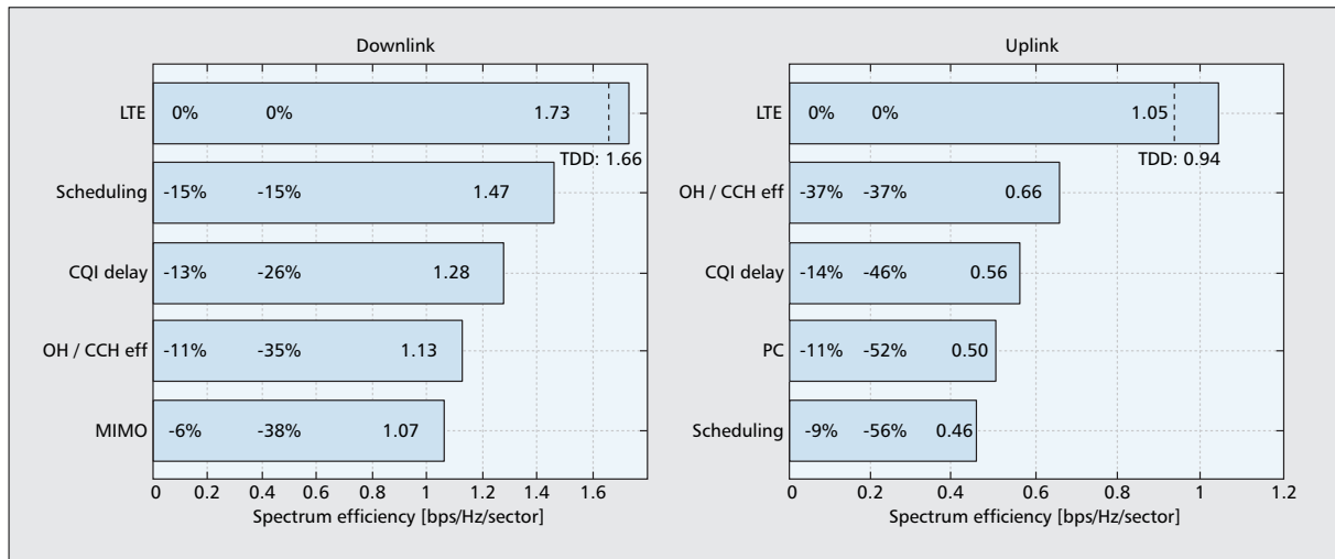
■ Figure 6. Spectrum efficiency in downlink and uplink.
