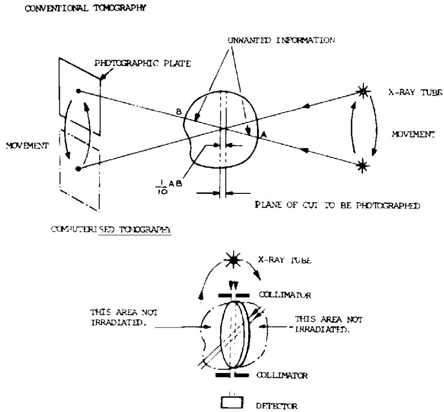
Fig. 9. Illustrating the improved efficiency of information collection when conventional tomography and CT are compared.
