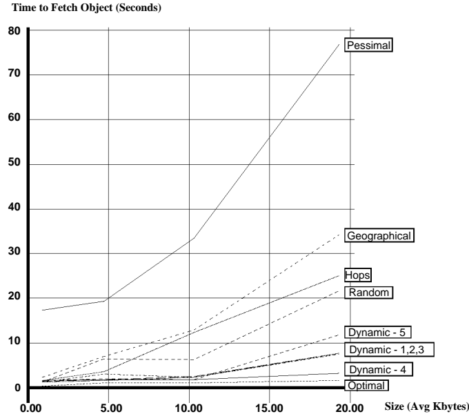
Figure 5: Fetch Times of Static and Dynamic Policies Plotted Against Document Sizes.
