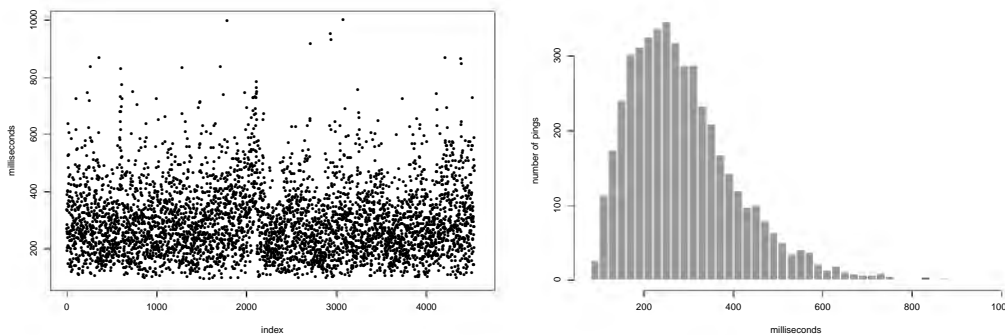
Figure 4: Round Trip Times to a Single Host
