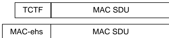
Figure 9.2.1.4.1: MAC PDU formats for CCCH
