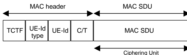
Figure 11.5.1: Cipherrered part unit for a MAC PDU
