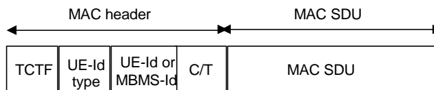
Figure 9.1.2.1: MAC PDU
