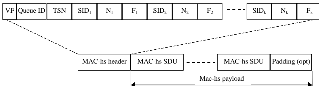
Figure 9.1.4.1: MAC-hs PDU
