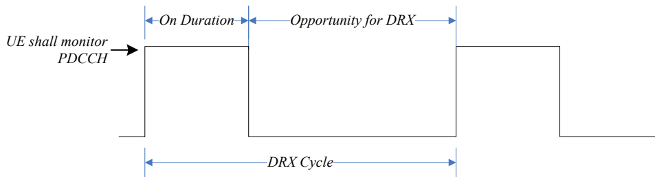
Figure 3.1-1: DRX Cycle
