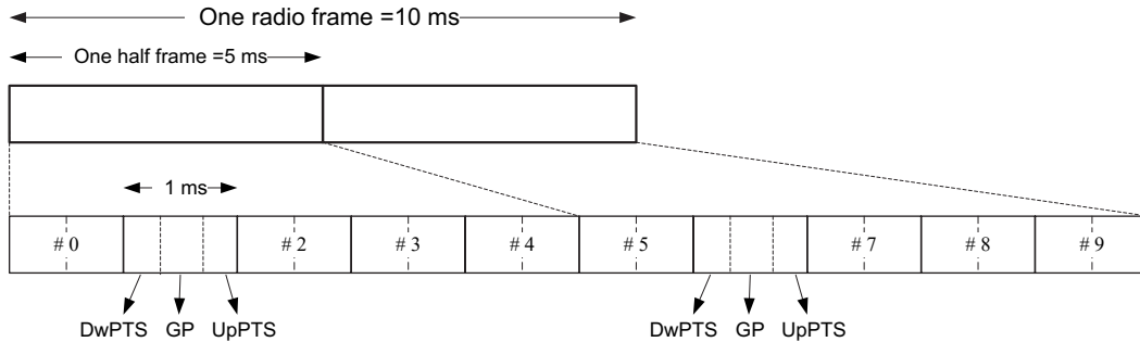
Figure 5.1-2: Frame structure type 2 (for 5ms switch-point periodicity)
