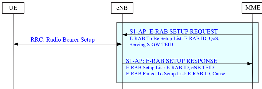
Figure 19.2.2.4.1-1: E-RAB Setup procedure
