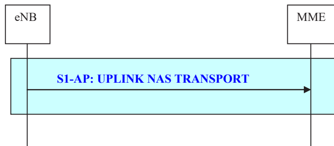
Figure 19.2.2.6-2: Uplink NAS Transport procedure
