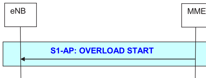
Figure 19.2.2.12.1-1 Overload Start procedure
