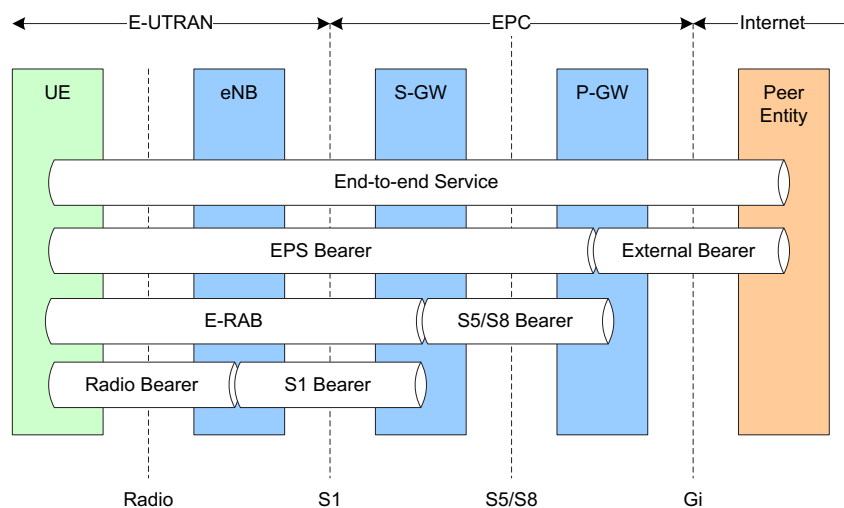
Figure 13.1-1: EPS Bearer Service Architecture
