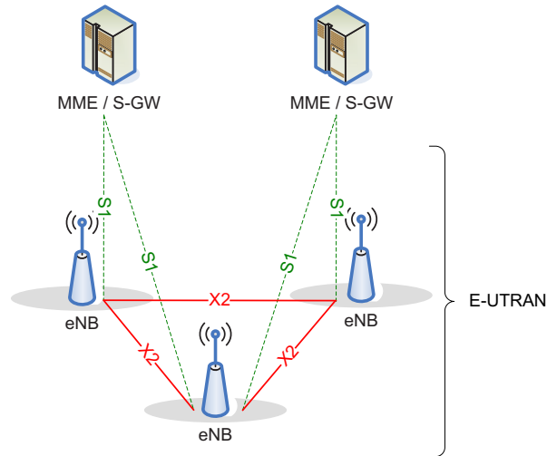
Figure 4-1: Overall Architecture
