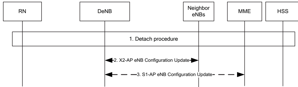
Figure 4.7.6.4-1: RN detach procedure
