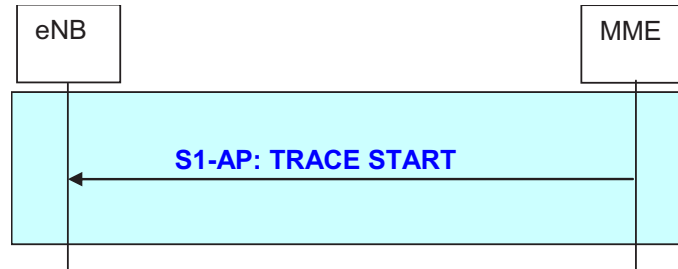
Figure 19.2.2.19.1-1: Trace Start procedure
