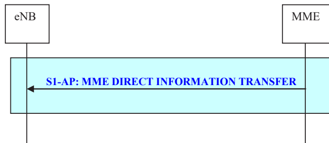
Figure 19.2.2.15-1: MME Direct Information Transfer procedure
