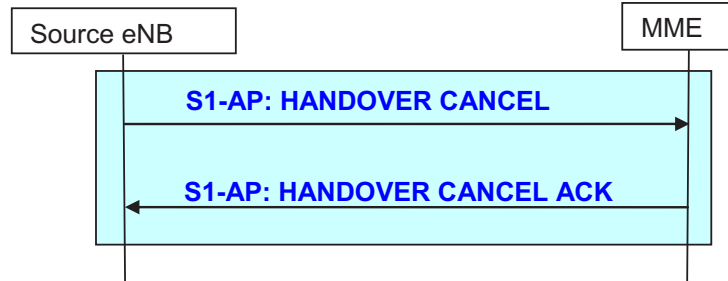
Figure 19.2.2.5.4-1: Handover cancellation procedure
