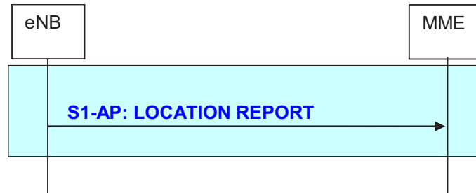
Figure 19.2.2.11.2-1: Location Report procedure
