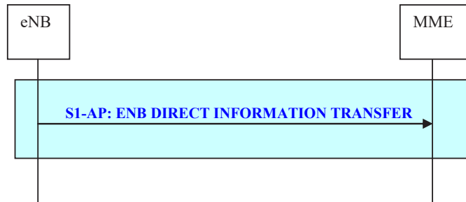
Figure 19.2.2.14-1: eNB Direct Information Transfer procedure
