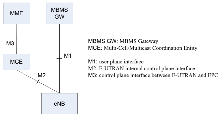
Figure 15.1.1-1: E-MBMS Logical Architecture
