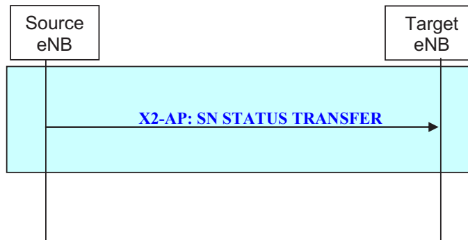
Figure 20.2.2.4-1: SN Status Transfer procedure
