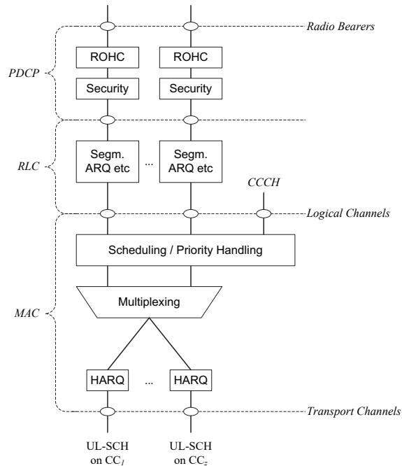
Figure 6.4-2: Layer 2 Structure for UL with CA configured
