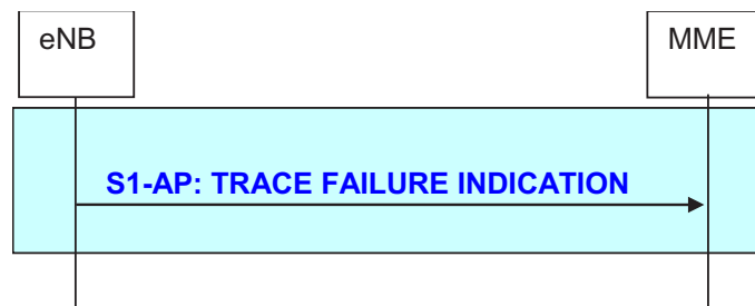
Figure 19.2.2.19.2-1: Trace Failure Indication procedure
