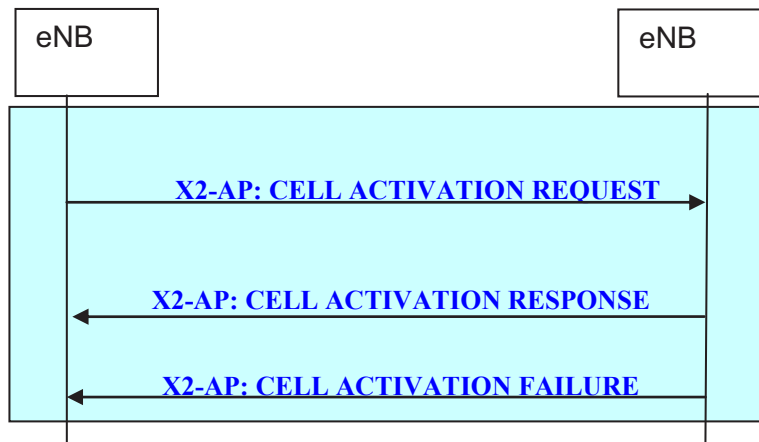
Figure 20.2.2.15-1: Cell Activation procedure
