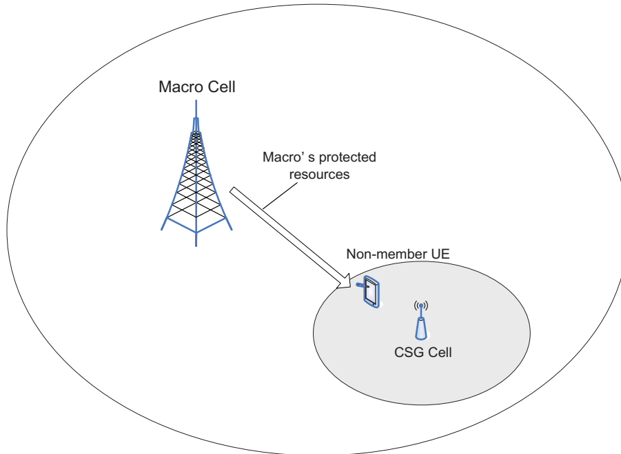
Figure K.1.1-1: Time domain ICIC: CSG scenario
