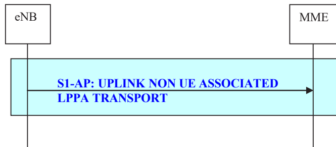
Figure 19.2.2.18.4-1: Uplink Non UE Associated LPPa Transport procedure
