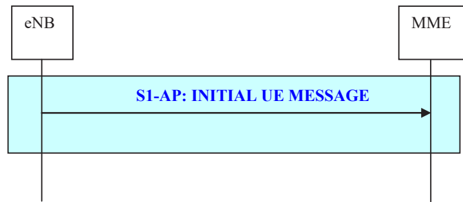
Figure 19.2.2.6-1: Initial UE Message procedure
