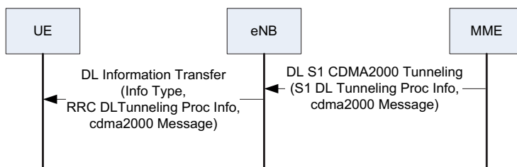
Figure 10.3.2.1-1: Downlink Direct Transfer
