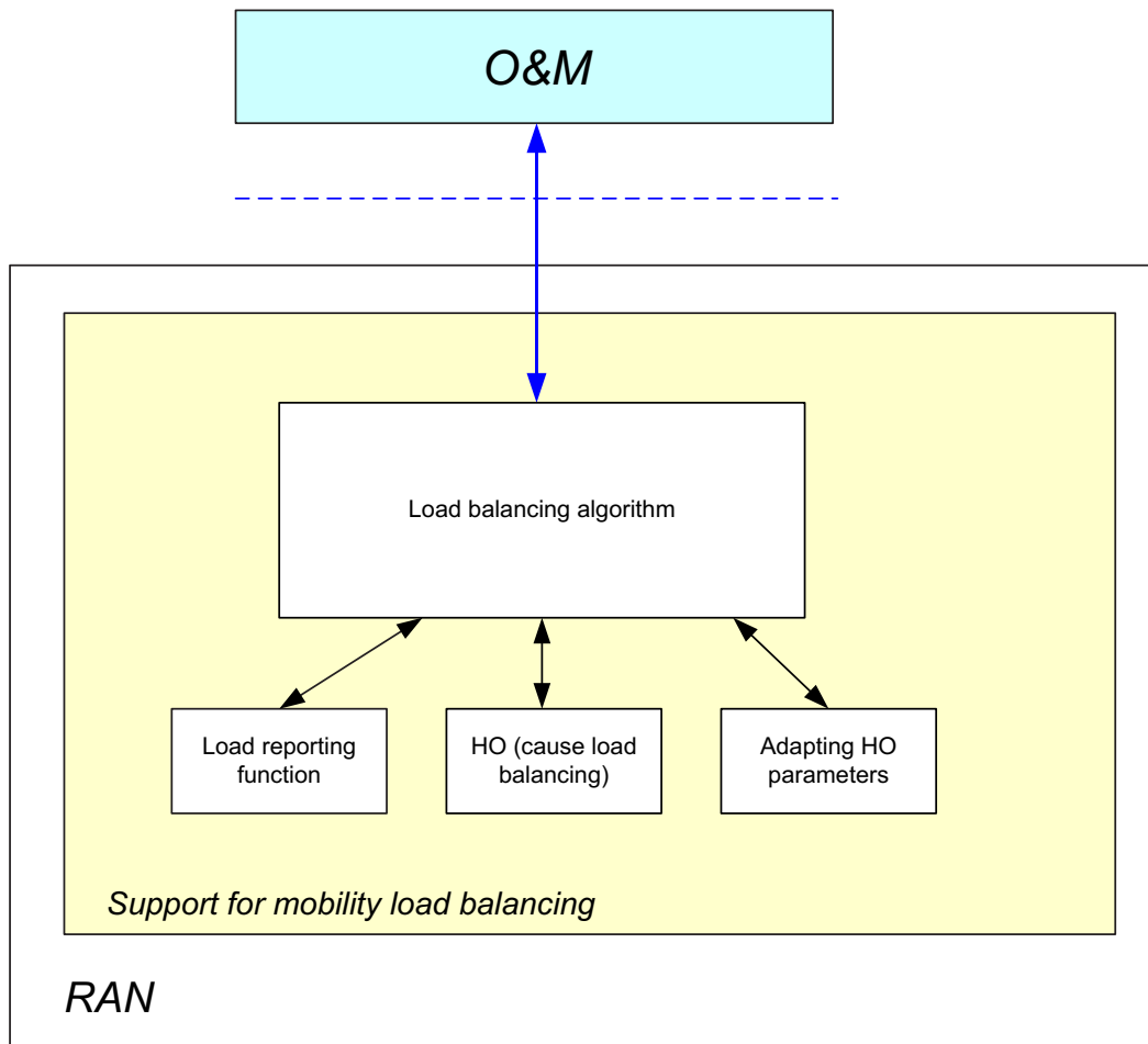
Figure 22.4.1.1-1: Functional architecture of SON load balancing
