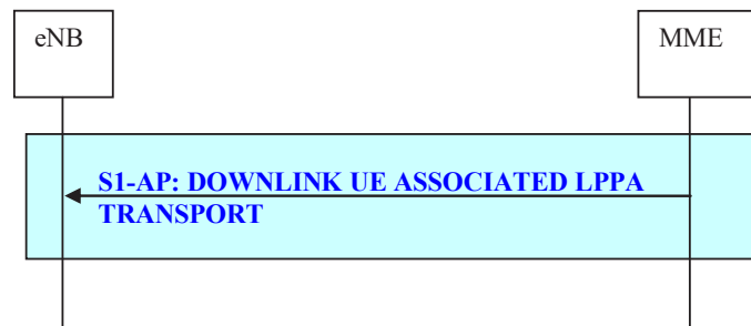
Figure 19.2.2.18.1-1: Downlink UE Associated LPPa Transport procedure
