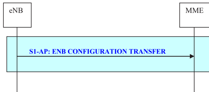
Figure 19.2.2.9a-1: eNB Configuration Transfer procedure
