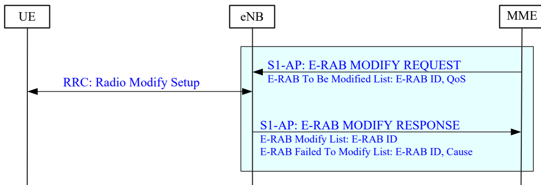
Figure 19.2.2.4.2-1: E-RAB Modification procedure
