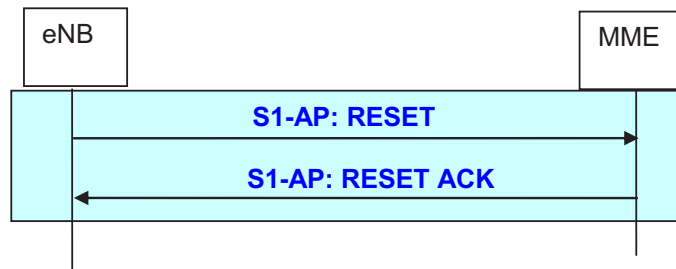
Figure 19.2.2.7.1a-1: eNB initiated Reset procedure
