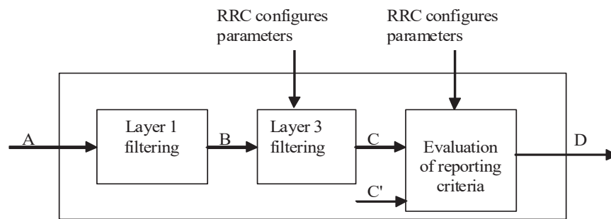
Figure 10.6-1: Measurement model
