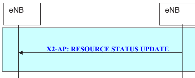
Figure 20.2.2.11-1: Resource Status Reporting procedure
