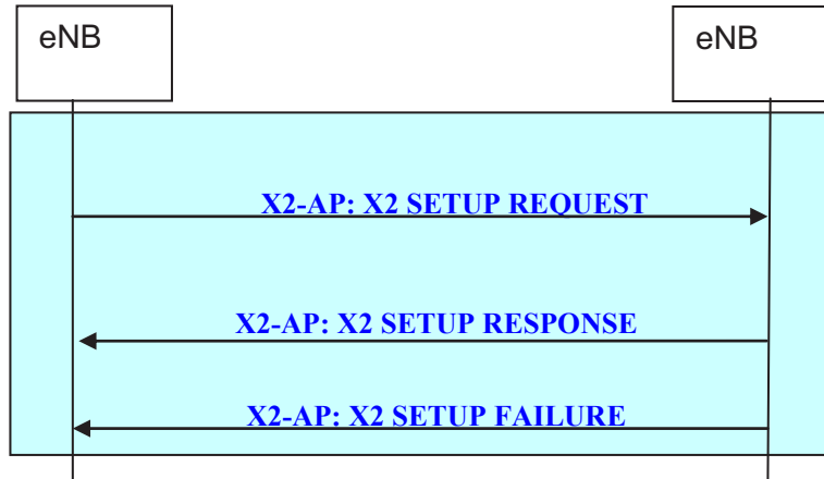
Figure 20.2.2.7-1: X2 Setup procedure
