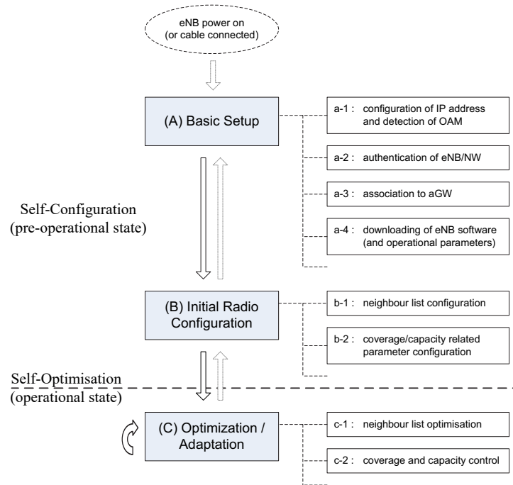
Figure 22.1-1: Ramifications of Self-Configuration /Self-Optimization functionality
