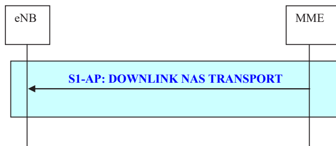
Figure 19.2.2.6-3: Downlink NAS Transport procedure
