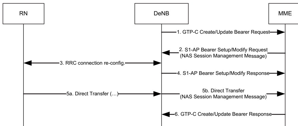
Figure 4.7.6.2-1: DeNB-initiated bearer activation/modification procedure
