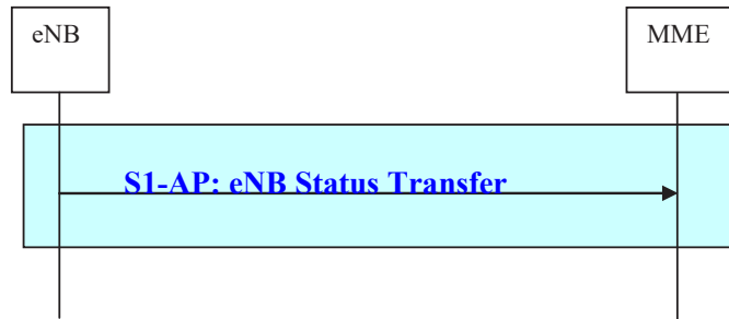
Figure 19.2.2.5.7-1: eNB Status Transfer
