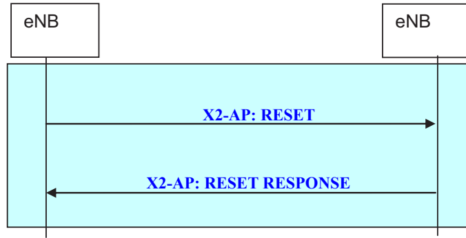
Figure 20.2.2.9-1: Reset procedure
