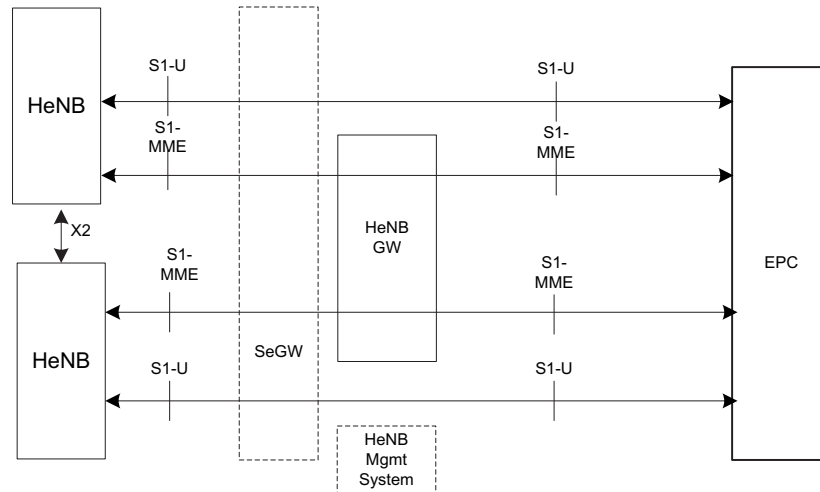
Figure 4.6.1-1: E-UTRAN HeNB Logical Architecture
