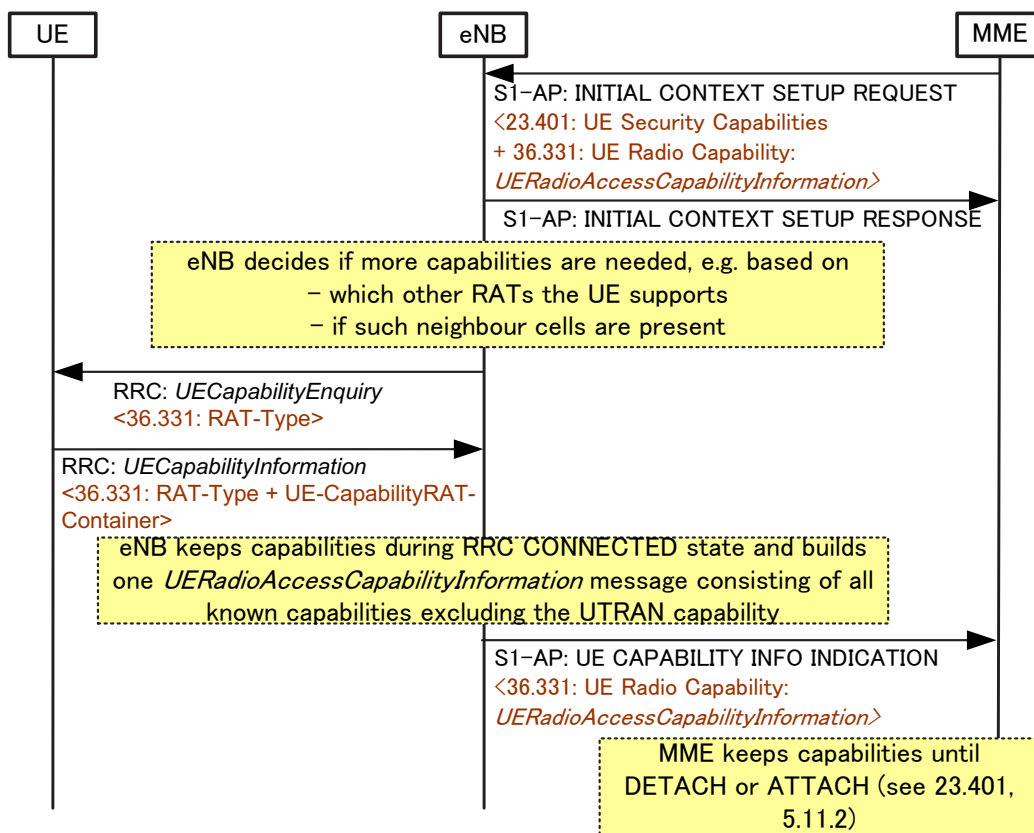
Figure 18-1: Initial UE Capability Handling
