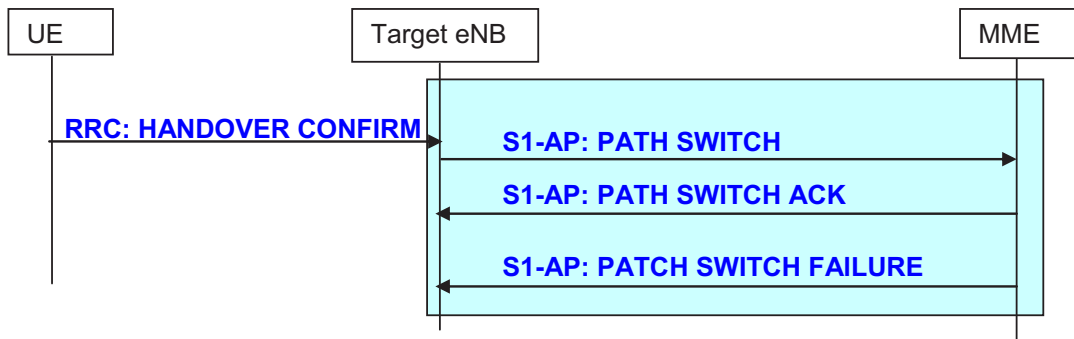
Figure 19.2.2.5.5-1: Path Switch procedure
