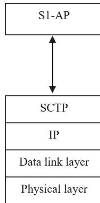
Figure 19.2-1: S1 Interface Control Plane (eNB-MME)
