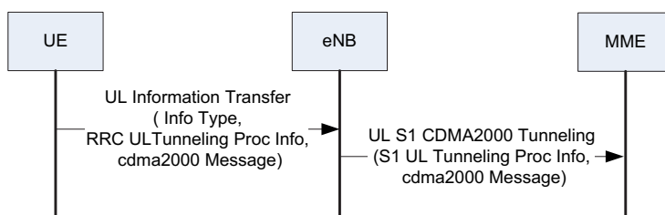
Figure 10.3.2.1-2: Uplink Direct Transfer
