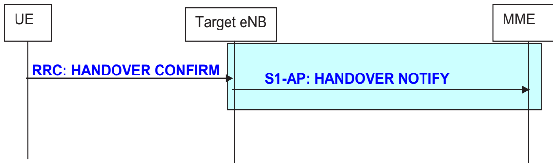
Figure 19.2.2.5.3-1: Handover completion procedure
