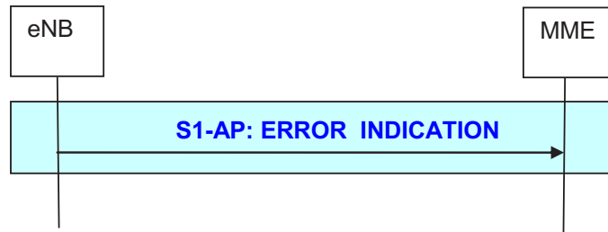
Figure 19.2.2.7.2a-1: eNB initiated Error Indication procedure
