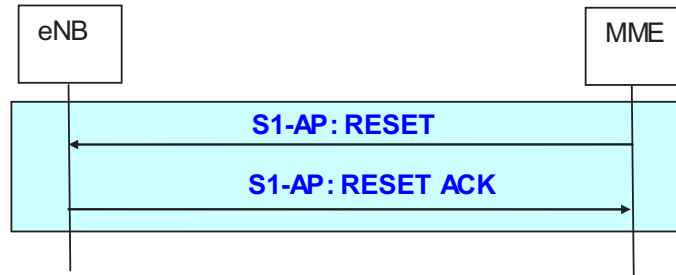
Figure 19.2.2.7.1b-1: MME initiated Reset procedure
