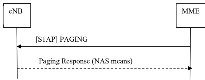
Figure 19.2.2.1-1: Paging procedure
