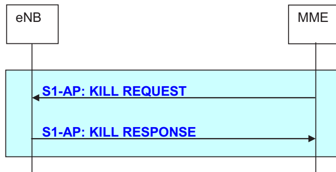
Figure 19.2.2.17-1: Kill procedure
