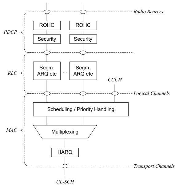
Figure 6-2: Layer 2 Structure for UL
