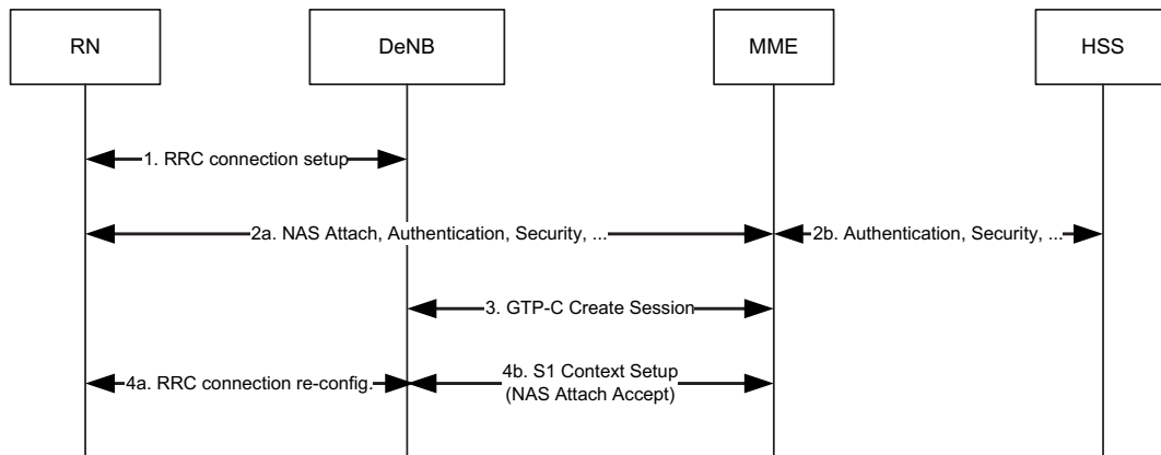
Figure 4.7.6.1-1: RN attach procedure
