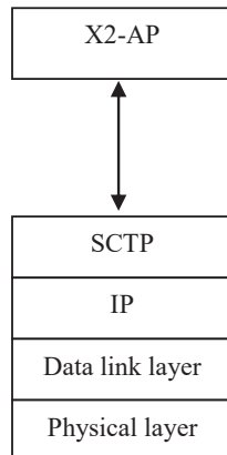
Figure 20.2-1: X2 Interface Control Plane
