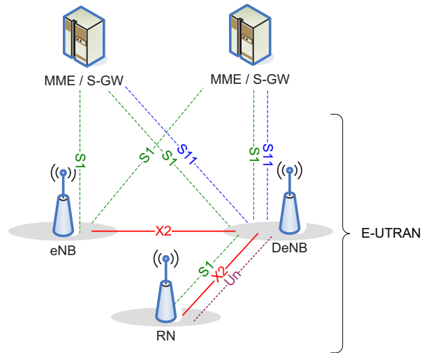
Figure 4.7.2-1: Overall E-UTRAN Architecture supporting RNs
