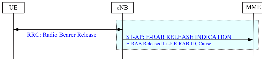
Figure 19.2.2.4.4-1: E-RAB Release Indication procedure
