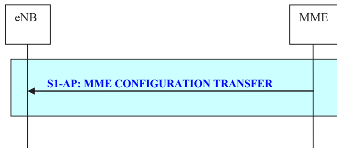
Figure 19.2.2.10a-1: MME Configuration Transfer procedure
