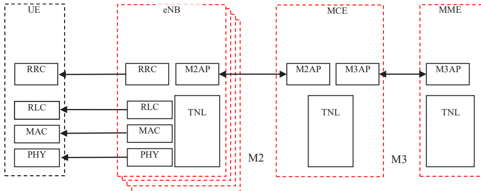
Figure 15.1.3-1: The E-MBMS c-plane architecture
