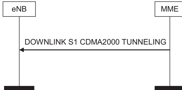
Figure 19.2.2.16.1-1: Downlink S1 CDMA2000 Tunnelling procedure
