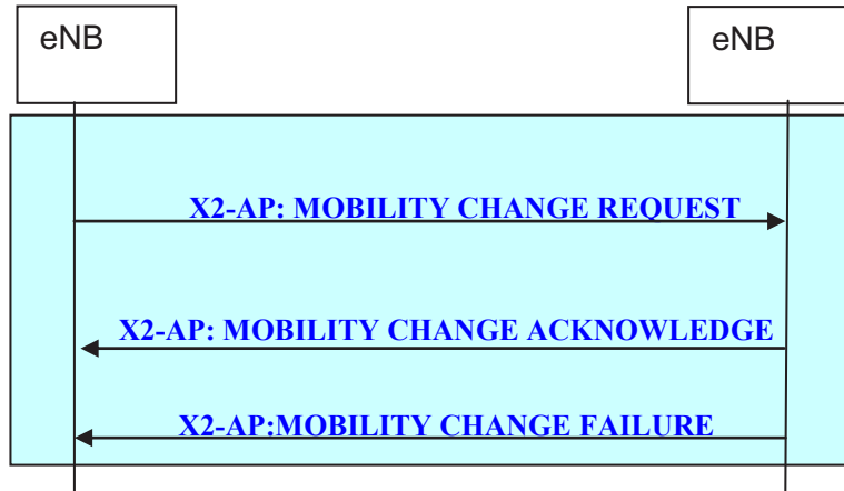
Figure 20.2.2.14-1: Mobility Settings Change procedure
