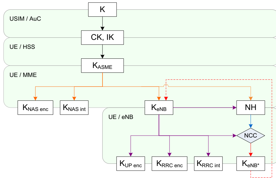
Figure 14.1-1: Key Derivation
