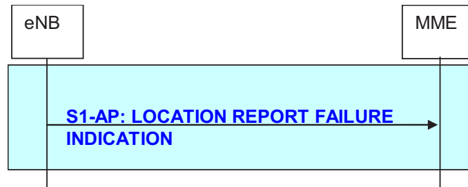
Figure 19.2.2.11.3-1: Location Report Failure Indication procedure
