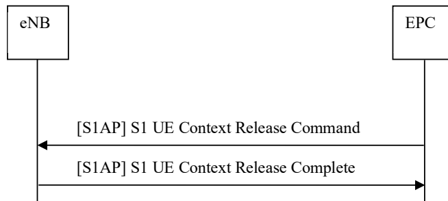
Figure 19.2.2.2.1-1: S1 UE Context Release procedure (EPC triggered)
