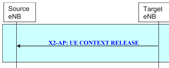
Figure 20.2.2.3-1: UE Context Release procedure
