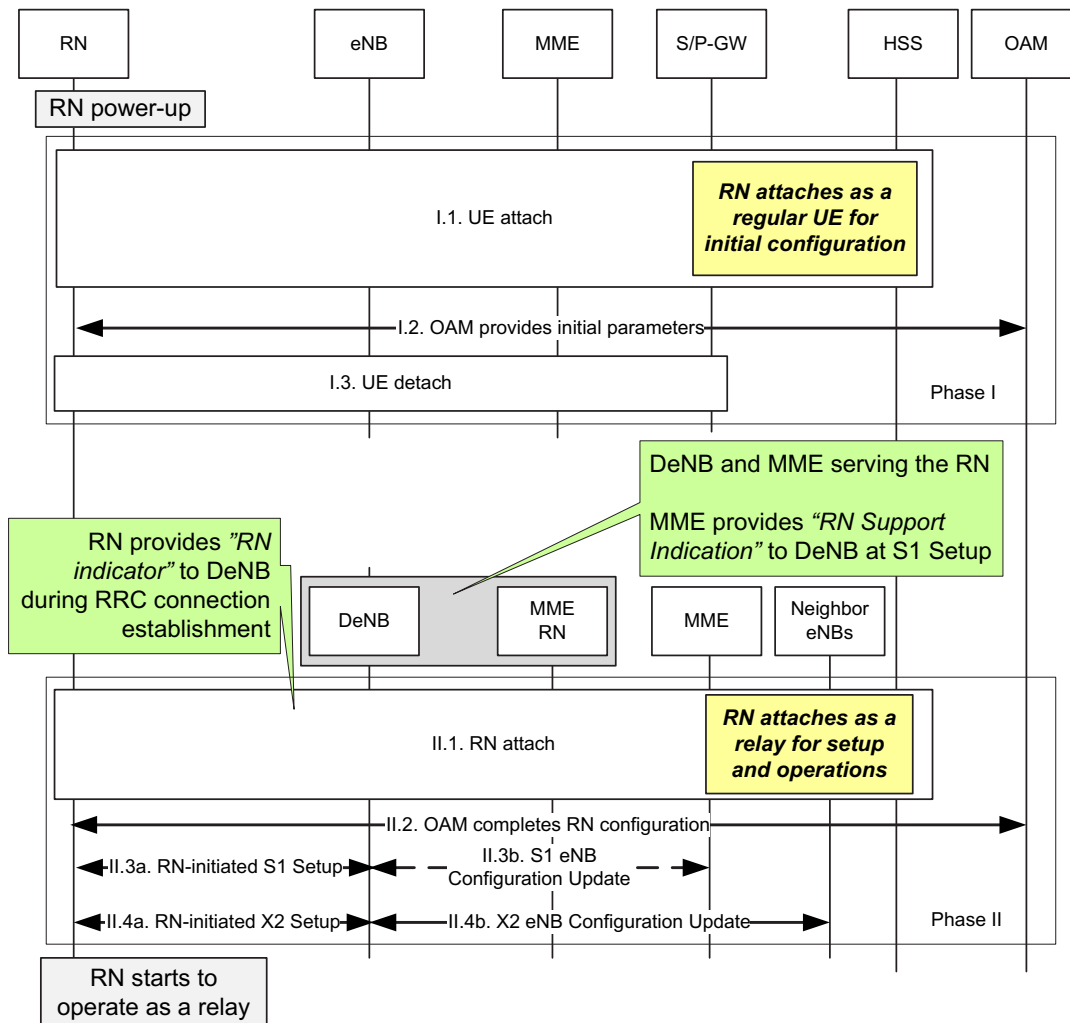
Figure 4.7.6.3-1: RN startup procedure
