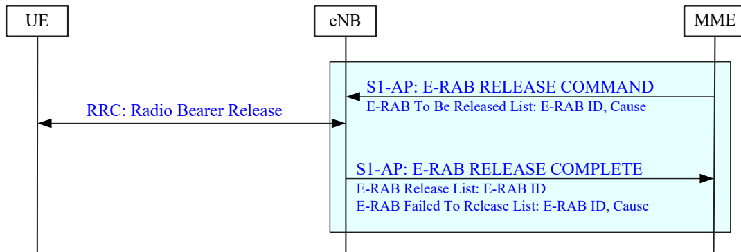
Figure 19.2.2.4.3-1: E-RAB Release procedure
