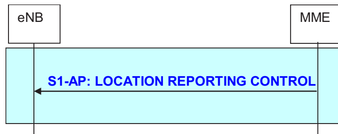
Figure 19.2.2.11.1-1: Location Reporting Control procedure
