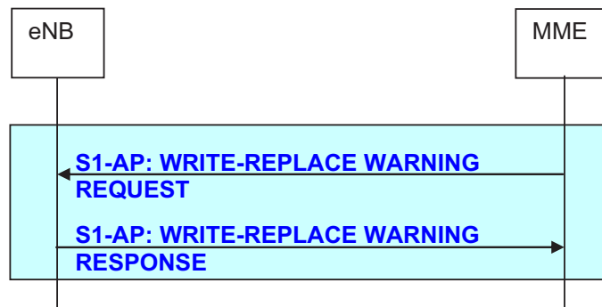
Figure 19.2.2.13.1-1: Write-Replace Warning procedure
