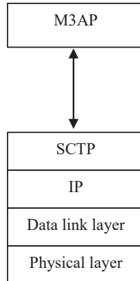
Figure 15.9.1-1: M3 Interface Control Plane (MME-MCE)
