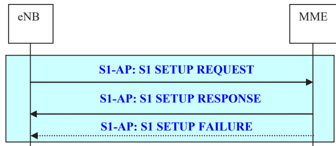
Figure 19.2.2.8-1: S1 Setup procedure
