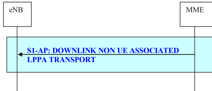
Figure 19.2.2.18.3-1: Downlink Non UE Associated LPPa Transport procedure
