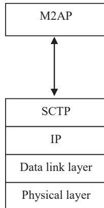
Figure 15.8.1-1: M2 Interface Control Plane (eNB-MCE)
