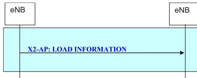
Figure 20.2.2.6-1: Load Indication procedure
