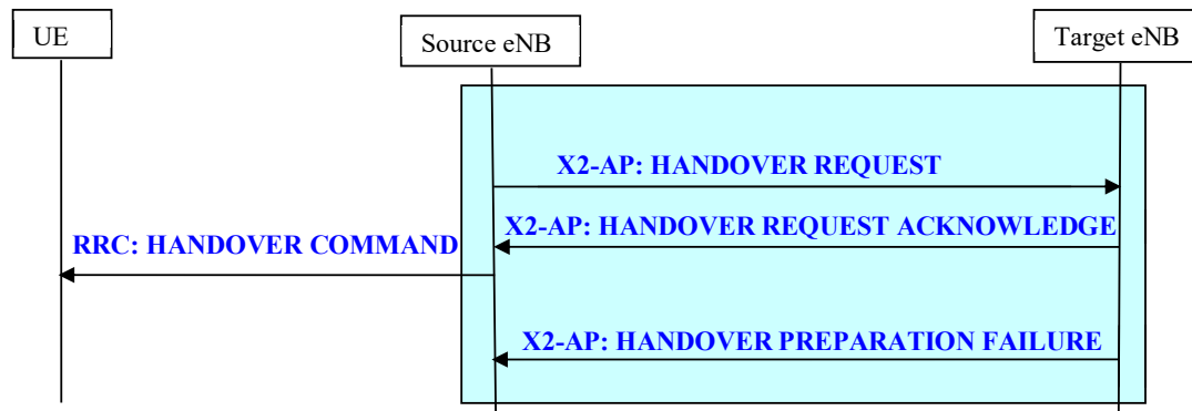
Figure 20.2.2.1-1: Handover Preparation procedure
