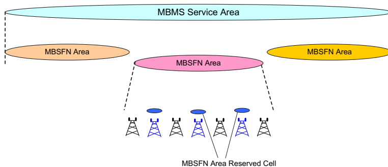
Figure 15-1: MBMS Definitions
