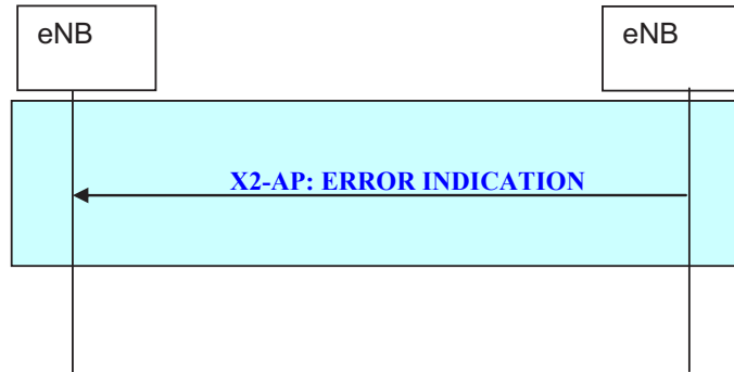
Figure 20.2.2.5-1: Error Indication procedure
