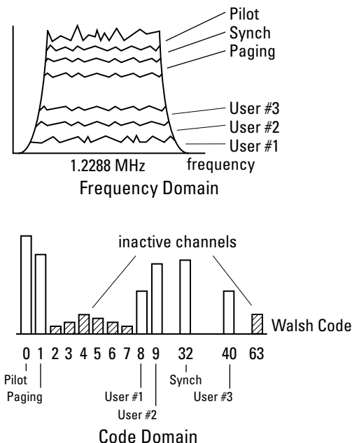
Figure 14. Code-domain power
