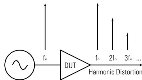
Figure 25. Harmonics
