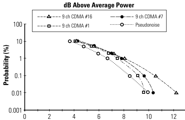
Figure 22. CDFs for three 9-channel signals with different traffic channels active
