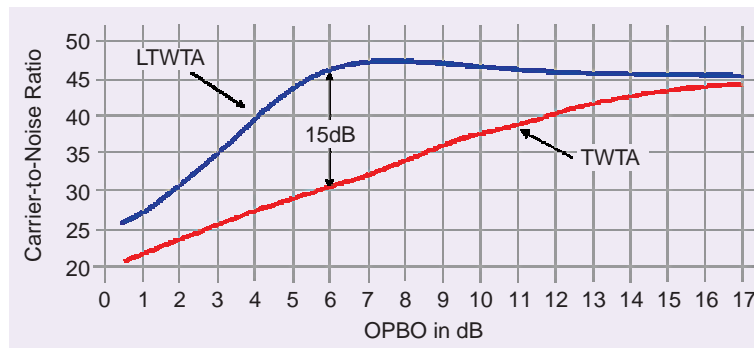
Figure 23. Reduction in spectral regrowth provided by linearization of a TWTA.
