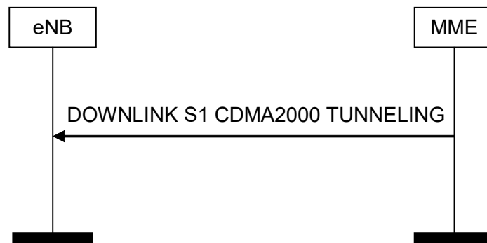
Figure 19.2.2.16.1-1: Downlink S1 CDMA2000 Tunneling procedure
