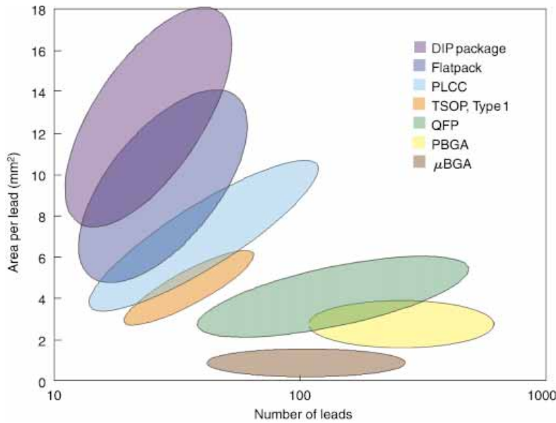
Figure 4. Plot showing the amount of substrate area required per lead and how this ratio varies with package style and total number of leads on the package. (DIP = dual-inline package, PLCC = plastic-leaded chip carrier, TSOP = thin small-outline package, QFP = quad flatpack, BGA = gall-grid array, PBGA = plastic BGA.)
