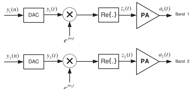
Fig. 1. Block diagram of multiple ratio system.
