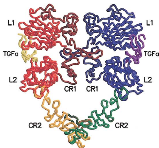
Fig. 3. Transforming growth factor- \alpha (TGF \alpha )-bound EGFR501 dimer with superimposed CR2 domains of ErbB3 [18–20]. Each of the proteins and protein domains are rendered as C_{\alpha} worms. The EGFR501 molecules are colored red and blue with their CR2 domains colored with darker tones; the bound TGF \alpha molecules are colored yellow and dark purple. The CR2 domains of ErbB3 were superimposed onto the epidermal growth factor (EGF) receptor fragments by using the C_{\alpha} atoms of the first module of the CR2 domains of each. The two ErbB3 CR2 domains are colored orange and green except for residues 572–582, which are colored in darker tones.
