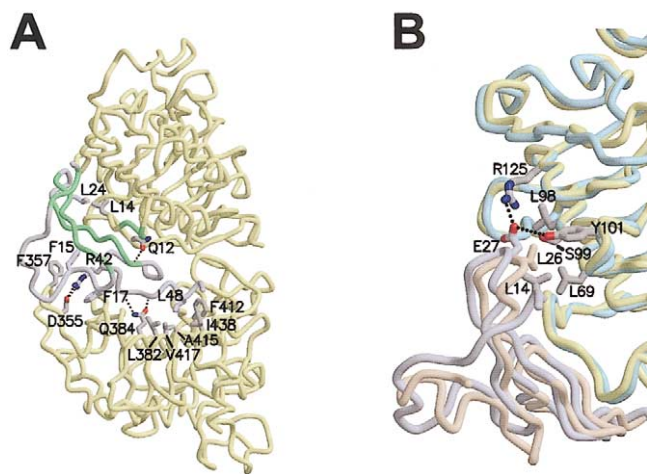
Fig. 2. Interactions between the epidermal growth factor (EGF) receptor (yellow) L1 and L2 domains with bound transforming growth factor- \alpha (TGF \alpha ) (metallic blue). Residues that contribute to a \beta -sheet that involves both the receptor and the ligand are colored green. The sidechains of selected ligand and receptor residues are shown as sticks. Selected hydrogen bonds are represented as dotted lines and mainchain atoms involved in these interactions are not rendered. (A) C_{\alpha} worm representation of TGF \alpha bound to the EGF receptor residue 1–501 [18] with a number of key interacting residues displayed. Carbon atoms of the sidechains of the EGF receptor are colored grey to increase their visibility. (B) Detail of interaction between TGF \alpha residue Glu 27 with the EGF receptor L1 domain. For comparison, the EGF receptor L1 domain (colored cyan) and EGF (dark pink) [19] are shown as superimposed on the TGF \alpha -bound EGF receptor structure. The sidechain of EGF residue corresponding to TGF \alpha Glu 27, Leu 26, is also rendered to illustrate how this residue can be accommodated by the receptor. This figure and Fig. 3 were created by using the programs Molscript [292] and Raster3D [293].
