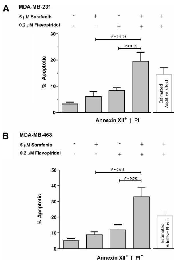
Figure 4. Potentiation of SFN-induced apoptosis by FPD. Cells were treated with either DMSO, 0.2 \mu M FPD, 5 \mu M SFN, or 1:25 ratio of FPD-SFN (0.2 \mu M and 5 \mu M, respectively) for 24 hours. The percentages (mean \pm SEM) of early apoptotic (annexin XII + ), non-necrotic (PI - ) MDA-MB-231 (A) and MDA-MB-468 (B) cells detected after drug treatment (gray bars) are shown. The white bar indicates the fraction of apoptotic cells expected by simple addition of the percentage of apoptotic cells induced by SFN or FPD alone. Significant P values are indicated ( t test; n = 3-4).
