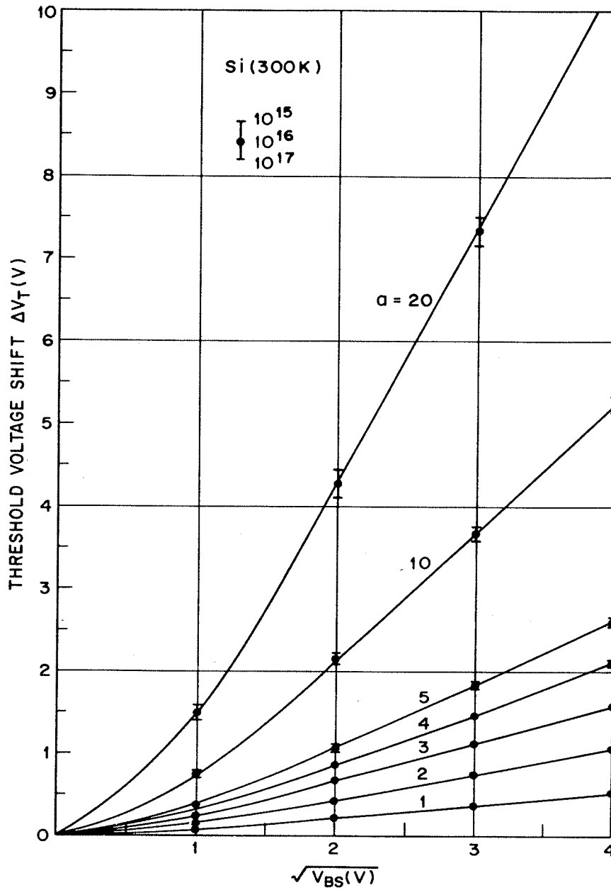
Fig. 9 Threshold voltage shift versus substrate reverse bias for various a values.
