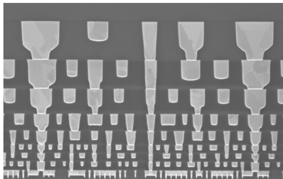
Figure 11: Cross-section of interconnect stack (8 layers)
