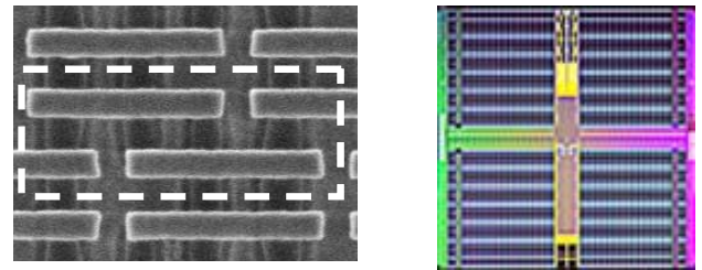
Figure 14: (a) diffusion and poly layers of 0.171 \mu\text{m}^2 SRAM and (b) 291Mb SRAM die photo
