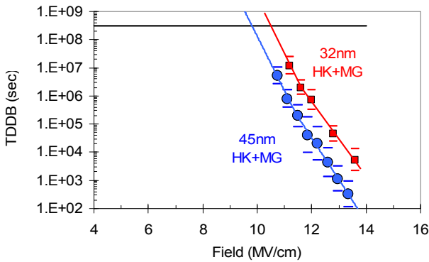
Figure 10: NMOS TDDF time-to-fail vs electric field
