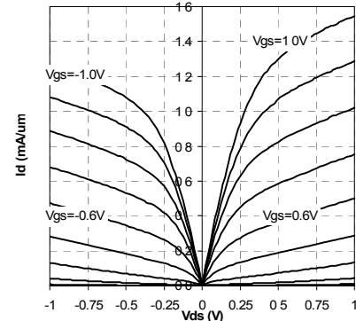
Figure 5: Transistor I-V curves
