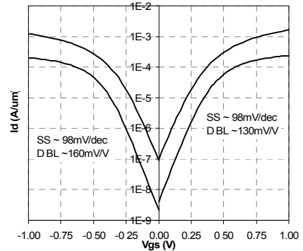
Figure 6: Sub-threshold curves
