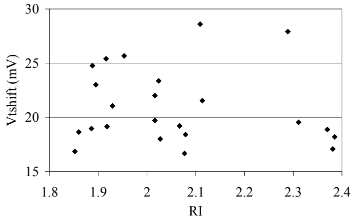
Figure14. Vt shift versus nitride film RI. No correlation.
