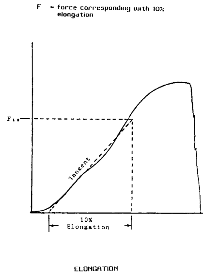
FIG. 2 Force-Elongation Curve for the Determination of Initial Modulus
