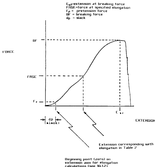
FIG. 1 Force-Extension Curve
