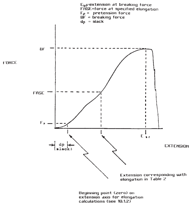
FIG. 1 Force-Extension Curve
