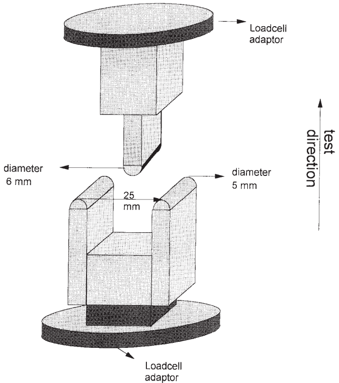
FIG. 5 Alternative Apparatus for Stiffness of Fabric Testing
