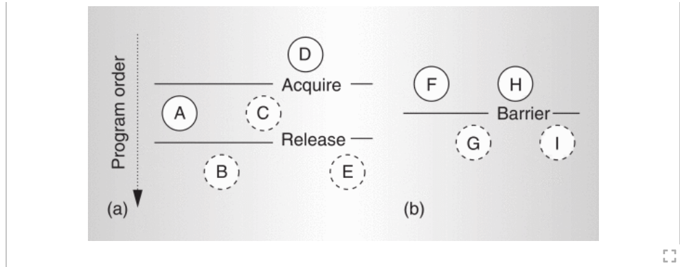
Figure 1. Example of a speculative lock (a) and barrier (b). Dashed and solid circles denote speculative and safe threads, respectively.
