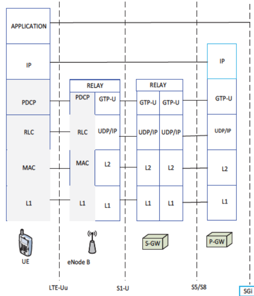
Fig. 3: LTE User Plane Protocol Stack
