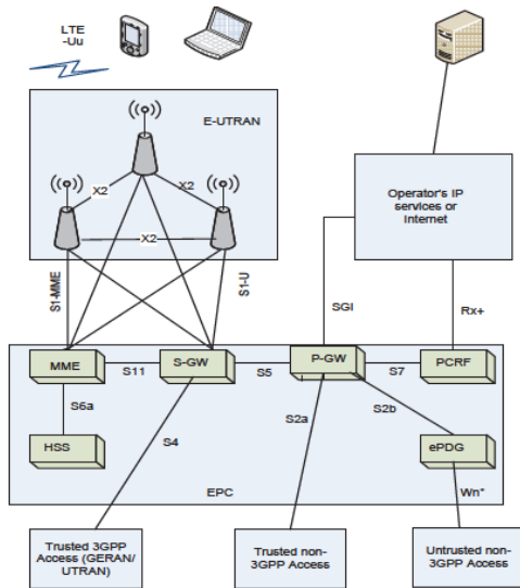
Fig. 1: EPS Network Elements
