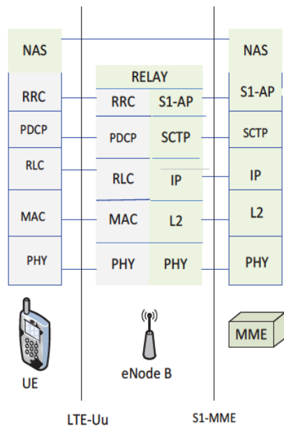
Fig. 2: LTE Control Plane Protocol Stack
